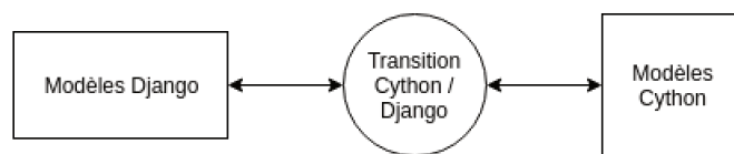
Figure 7.3 – Interaction Django/Cython
