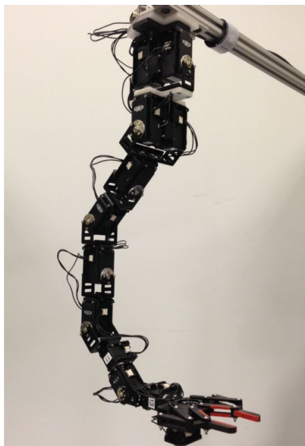
FIGURE 2.3: 6 DoF hyper-redundant manipulator for Mobile Manipulating UAVs [3]
