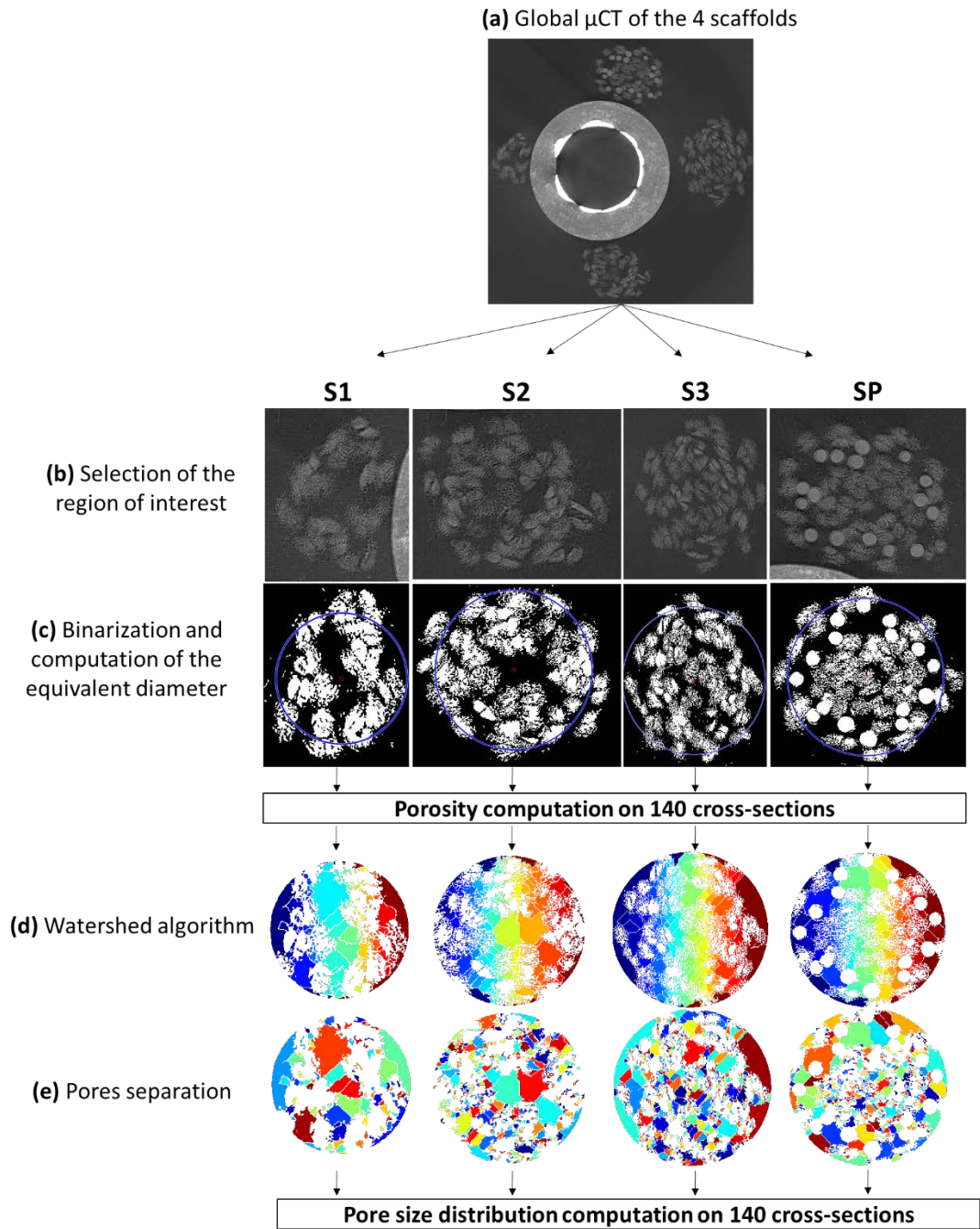
Figure 8 The flow chart of \mu -CT results post-treatment for silk and silk/PLCL scaffolds (S1: one-layer silk scaffold; S2: two-layer silk scaffold; S3: three-layer silk scaffold; SP: silk/PLCL composite scaffold)
