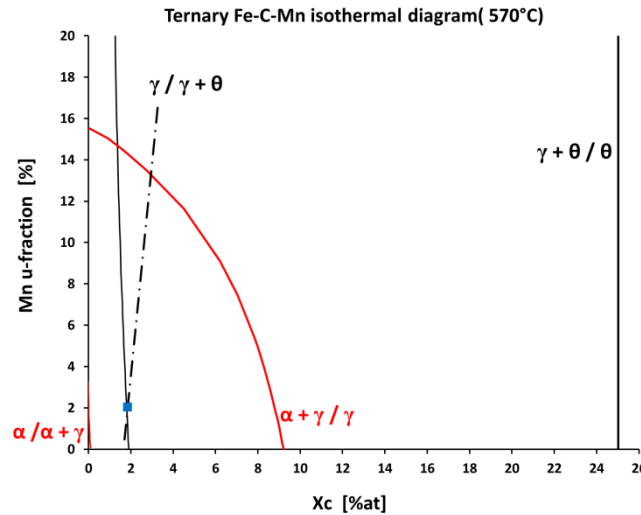
Figure 3.11: Isothermal section of the Fe-C-Mn diagram at 570°C. The dotted-dashed line represents the carbon iso-activity determined from the austenite bulk composition. The two domains delimited by the red and black boundaries represent respectively the \alpha + \gamma and \theta + \gamma two-phase fields.
