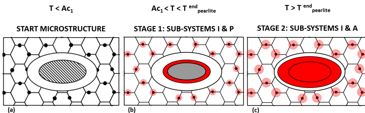
Figure 5.16: Scheme of the geometrical representation of the microstructure: sequence of the austenite transformation.
