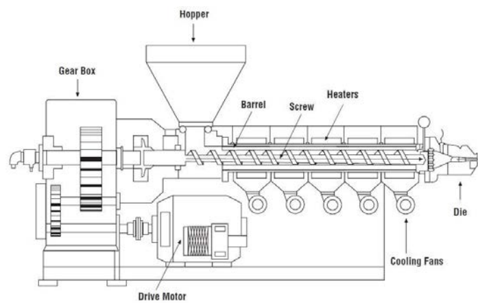
Figure 1-35. Single Screw Extruder [221]
