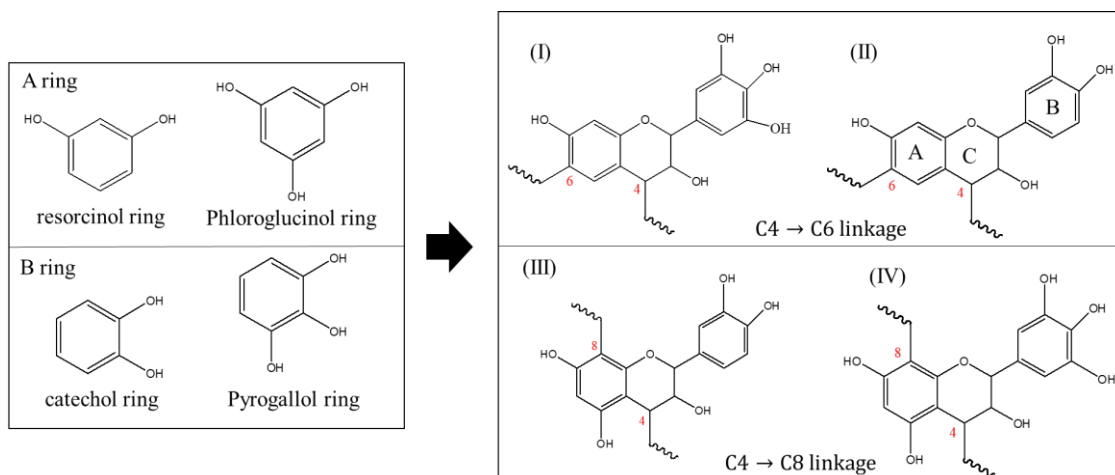
Figure 1-2. Structure of four main nonflavonoid building blocks. Linkage between flavonoid units: C4→C6(I)(II); C4→C8(III)(IV) (modify from reference [8,11])
