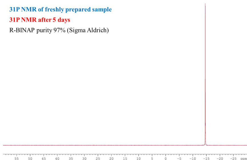
Figure 2.7: ^{31}\text{P} – \text{NMR} of 2 wt.% R-BINAP dissolved in toluene (with sensitivity correction), before and after five days of solution preparation.
