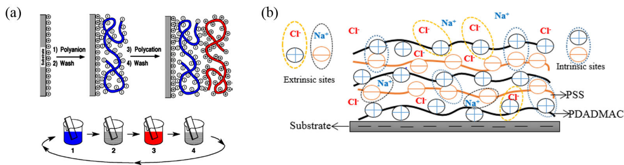
Figure 1.16: (a) LbL deposition via dip coating (Decher, 1997). (b) Scheme of intrinsic and extrinsic charge balance in the polyelectrolytes multilayer (PEM), adopted from (Ghostine et al., 2013)
