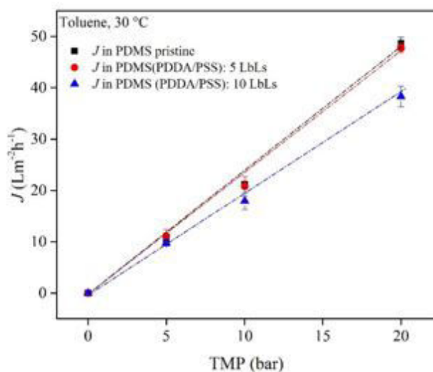
Figure 3. Effect of number of bilayers (PDPA/PSS) in toluene OSN fluxes (30 °C)
