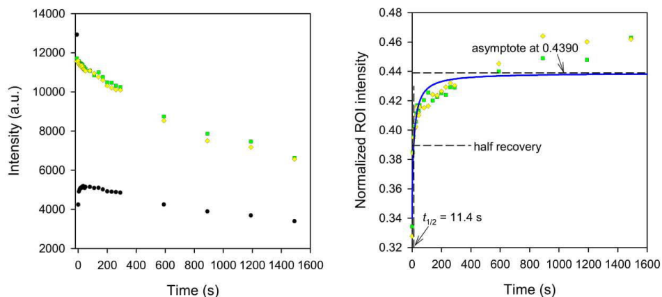
Figure 8. (PAH/PAA) 10 film on PDMS. Left panel: Raw fluorescence intensity in the ROI (black) and the two reference areas (green, yellow). Right panel: Normalized intensity in the ROI and graphical representation of eq. 4 (blue line) with optimized fitting parameters.
