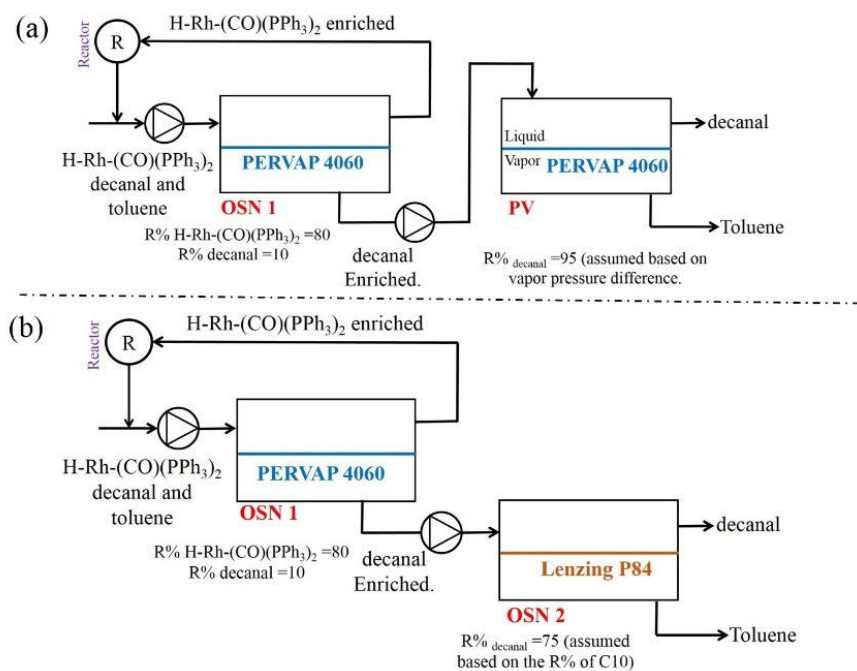
Figure 5.17: Scheme of OSN hybrids for the separation of catalyst and product from a hydroformylation system: (a) Hybrid OSN with PV. (b) Hybrid OSN using a dual membrane in series.
