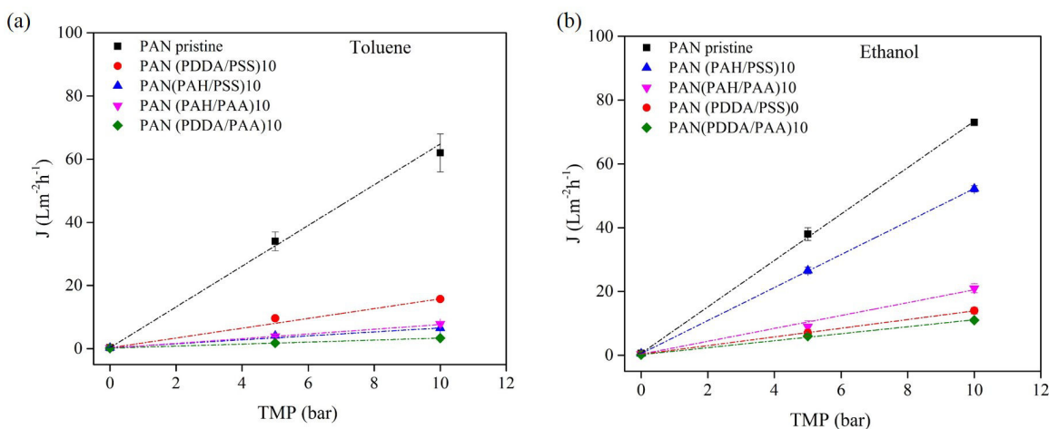
Figure 4.14: Comparison of pure solvent fluxes in pristine and PEM modified PAN membranes at 30°C, up to 10 bar using feed cross-flow 7 – 10 kg/h : (a) Toluene fluxes (b) EtOH fluxes.
