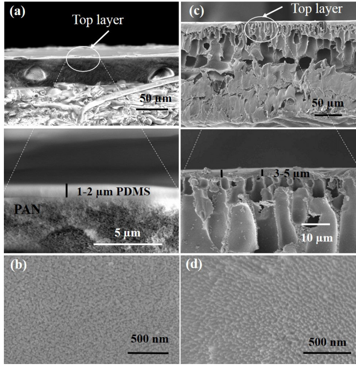
Figure 2.2: Microscopic images of dense membranes: (a) Cross-section and (b) surface of PERVAP 4060 (c) Cross-section and (d) surface of SOLSEP 010206.
