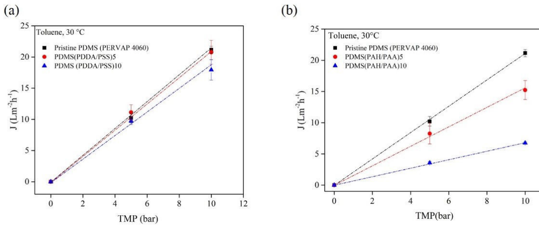
Figure 3.23: Effect of bilayers number on toluene permeation using (a) PDDA/PSS (b) PAH/PAA on PERVAP4060 at 30°C and 10 – 14 kg/h tangential flow.
