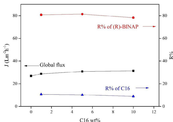
Figure 10. OSN performance of PERVAP4060 for the separation of a model ternary mixture consisting of C16 (1 to 10 wt%) and R-BINAP (0.05 wt%) in toluene (10 bar, 30^\circ\text{C} ). Deviation on J : \pm 10\% . [Color figure can be viewed at wileyonlinelibrary.com ]
