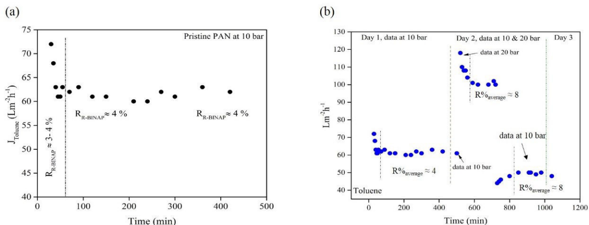
Figure 4.9: Toluene flux and R-BINAP rejection by pristine PAN in a long run study at 10 and 20 bar, 30°C and 7 – 10 kg/h cross-flow rate: (a) OSN measurement at 10 bar in day 1 (b) OSN measurement at 10 and 20 bar up to day 3
