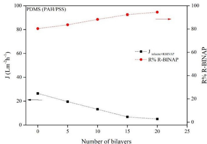
Figure 3.28: Effect of the number of bilayers on toluene flux, and R-BINAP rejection at 10 bar, 30°C and 7 – 10 kg/h cross-flow of diluted R-BINAP (0.05wt%) in toluene.
