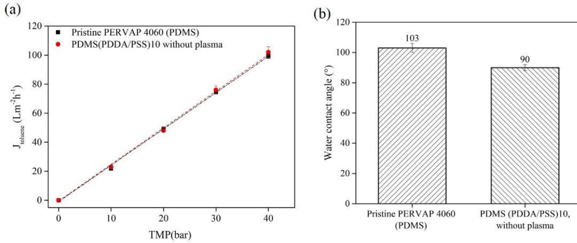
Figure 3.22: Effect of PDDA/PSS of 10 bilayers deposited on PDMS based PERVAP4060 without any plasma: (a) toluene permeation up to 40 bar at 30°C with 10–14 kg/h tangential flow. (b) Water contact angles before and after modification without using any intermediate plasma.
