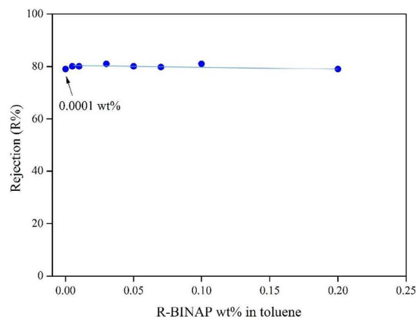
Figure 9. Evaluation of the effect of the concentration of the solute in toluene on its retention by PERVAP4060 (10 bar, 30^\circ\text{C} , concentration range: 0.0001–0.2 wt%). Deviation on rejection data: \pm 2\% . [Color figure can be viewed at wileyonlinelibrary.com ]
