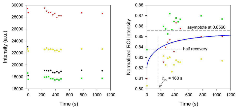
Figure 9. (PDDA/PAA) 10 film on PDMS. Left panel: Raw fluorescence intensity in the ROI (black) and the three reference areas (red, green, yellow). Right panel: Normalized intensity in the ROI and graphical representation of eq. 4 (blue line) with optimized fitting parameters.
