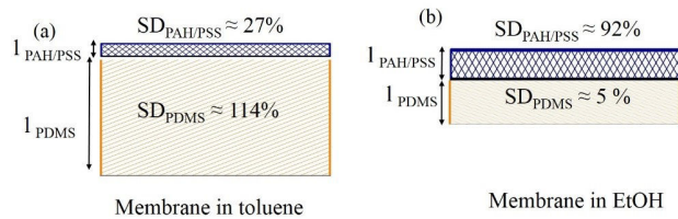
Figure 3.25: Global swelling of prototype membranes in (a) Toluene (b) EtOH. The swelling of PAH/PSS in toluene is adopted from (Ferrell et al., 2017), considering the PSS swelling.
