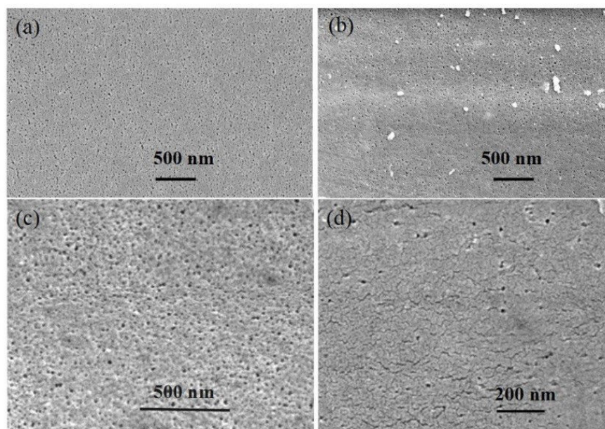
Figure 4.10: Surface of pristine PAN membrane: (a) and (c) before OSN (b) after OSN at 10 bar (d) after OSN at 20 bar; at 30°C and 7 – 10 kg/h cross-flow rate.
