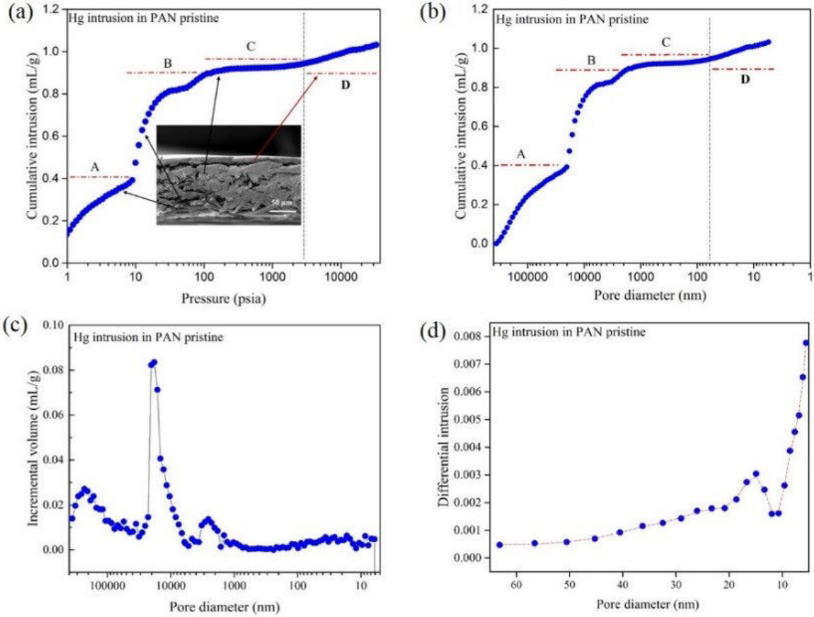
Figure 4.17: Mercury porosimetry for pristine PAN (a) Cumulative intrusion vs pressure plot. (b) Cumulative intrusion vs pore size (diameter). (c) Incremental volume and pore diameter (d) Differential intrusion vs diameter distribution.
