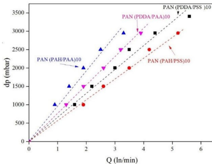
Figure 4.16: Air permeability measurement in PAN modified membranes.
