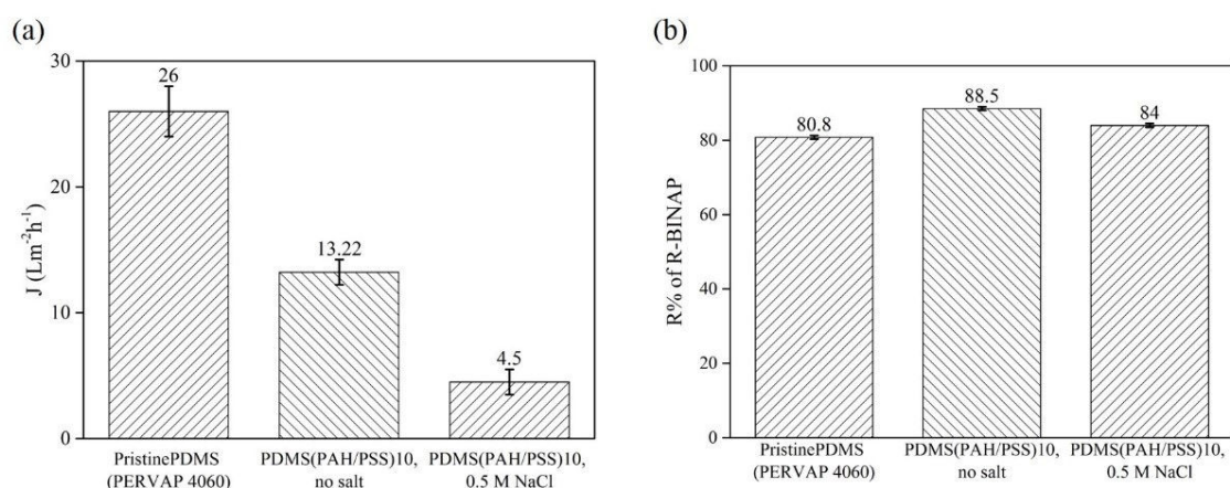
Figure 3.29: Effect of using salt in polyelectrolyte multilayer PEM preparation on PERVAP 4060; in terms of (a) toluene flux (b) R-BINAP rejection, at 10 bar, 30°C and 7 – 10 kg/h cross-flow of dilute R-BINAP (0.05wt%) in toluene.
