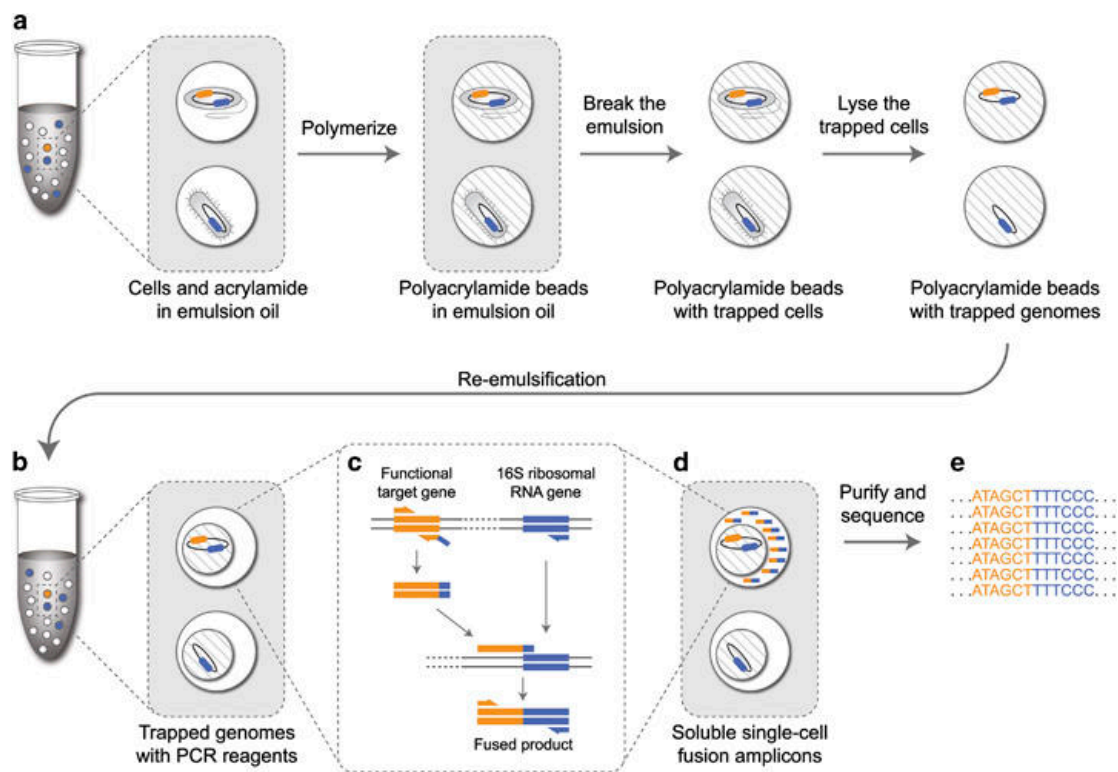
Figure 14 : Principe de l'epicPCR (Emulsion, Paired Isolation and Concatenation PCR) (Spencer et al., 2016).
