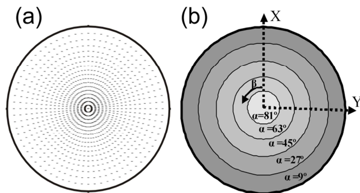
Fig. 1.1 Schemes of pole figure scan with (a) discrete method using an equal angular 5^\circ \times 5^\circ and (b) with discrete steps in \chi ( 0 \sim 90^\circ ) and continuous scanning of \varphi ( 0 \sim 360^\circ ).
