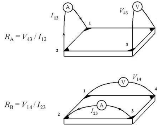
Figure 3.7 The principle of Van der Pauw's measurement
