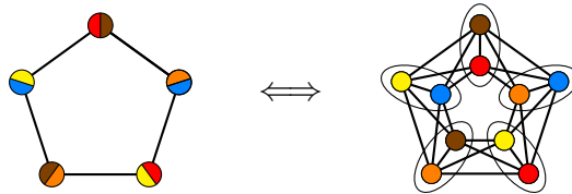
Figure 0.2.4: A proper (5 : 2) -colouring of C_5 , equivalent to a 5-colouring of C_5 \boxtimes K_2
