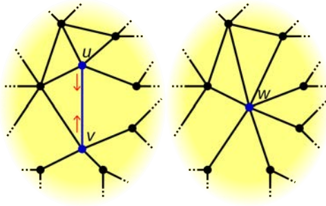
Figure 0.1.16: An illustration of edge contraction.
