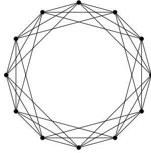
Figure 0.1.22: The distance-3 graph of the dodecagon C_{12}
