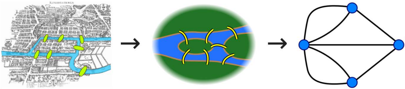
Figure 0.3.1: The multigraph representation of the seven bridges of Königsberg
