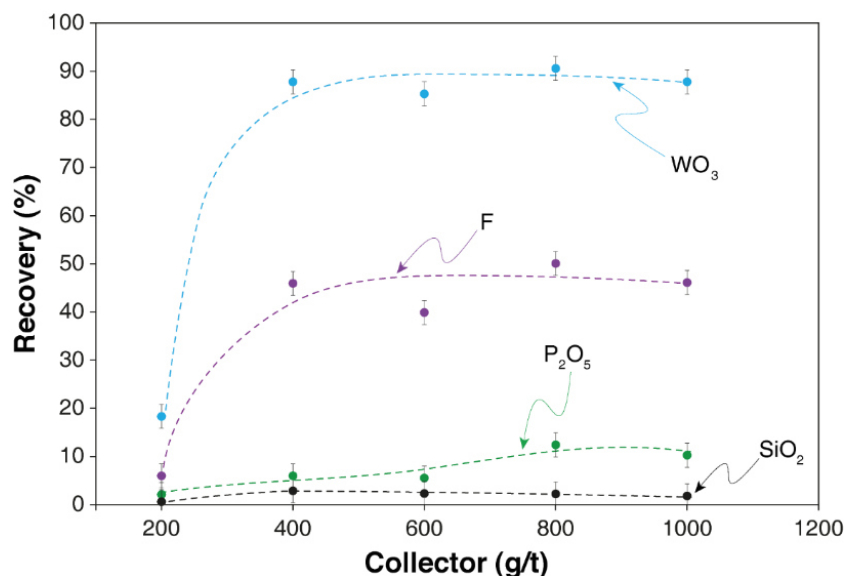
Figure 68. F, P 2 O 5 , SiO 2 , and WO 3 recoveries versus LD dosage.
