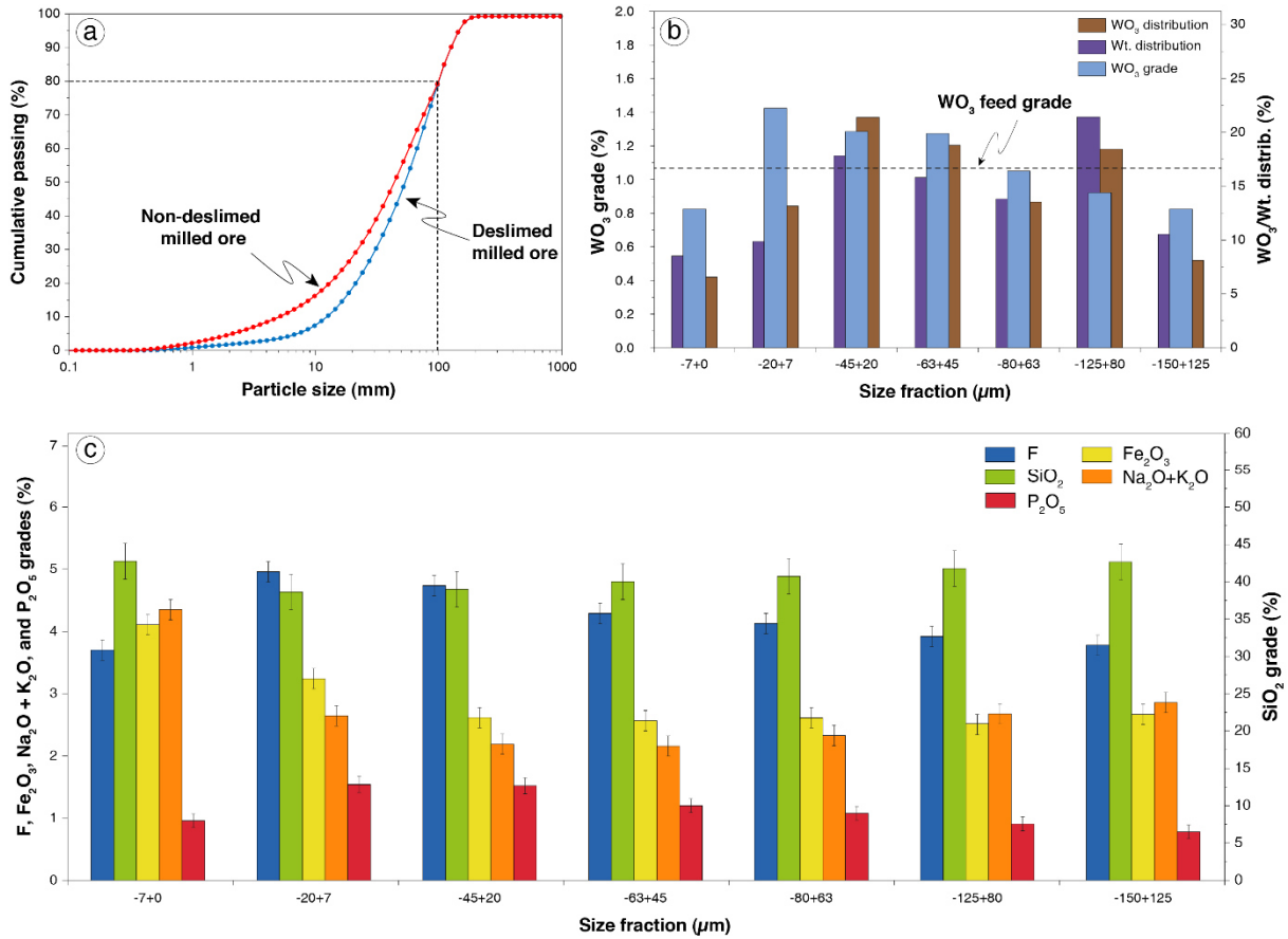
Figure 29. a. PSD of the Main Skarn Tabuaço ore after the milling stage, for the deslimed ore and the non-deslimed ore (used for Falcon tests). The dashed line shows the d_{80} of the two products. b. WO 3 grade, WO 3 distribution, and wt.% retained for each size fraction of the milled product (-150+0 μm). Since the WO 3 grade was measured by ICP-MS, the error bars are not displayed considering the accuracy of this method. c. F, SiO 2 , Fe 2 O 3 , Na 2 O + K 2 O, and P 2 O 5 grades in each size fraction of the milled ore, assessing the distributions of the main gangue minerals in the different size fractions. The error bars represent the average error claimed for each analysis method (ISE for F, ICP-AES for the other), which is roughly equivalent to 5% of the given value. For b and c , the -7+0 μm product corresponds to the hydrocyclone overflow when the ore was deslimed.
