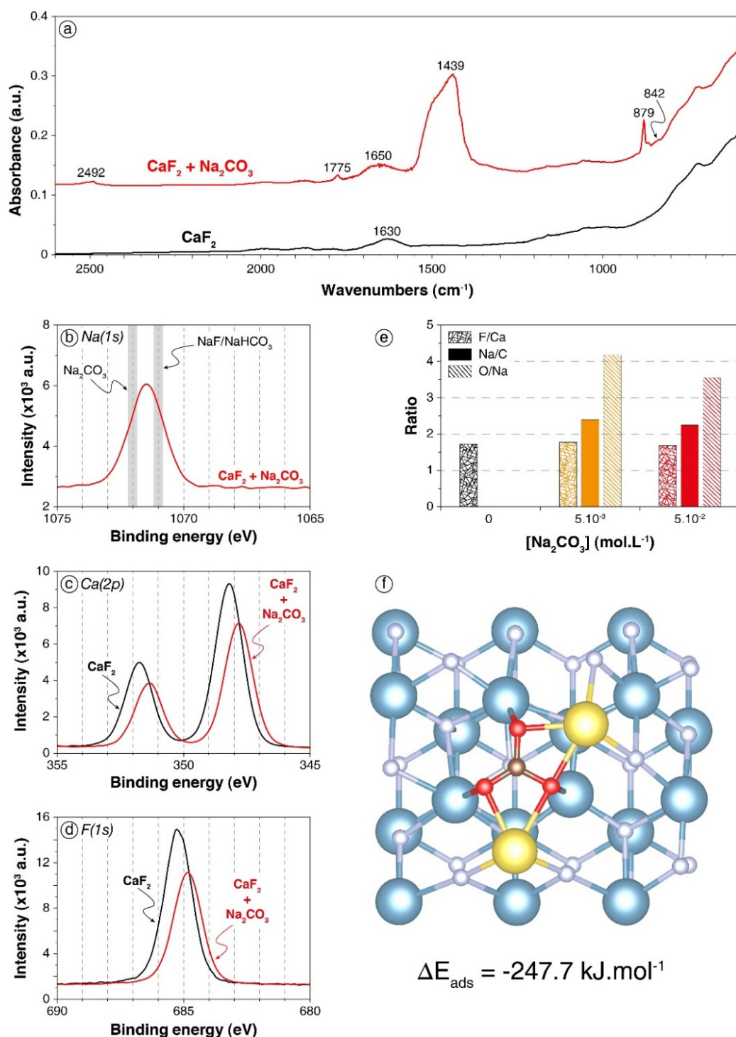
Figure 54. Carbonation of CaF 2 surface by Na 2 CO 3 addition. Black and red IR/XPS spectra represent pure CaF 2 conditioned in deionised water or in a 5.10 -2 mol.L -1 Na 2 CO 3 solution, respectively. a. DRIFT spectra b. XPS Na(1s) spectrum, with the common binding energies of Na-O and Na-F bonds [from (Briggs, 1981)]. c. XPS Ca(2p) spectra. d. XPS F(1s) spectra. e. F/Ca, Na/C, and O/Na ratios of CaF 2 conditioned in deionised water (black), in a 5.10 -3 mol.L -1 Na 2 CO 3 solution (orange), and in a 5.10 -2 mol.L -1 Na 2 CO 3 solution (red). f. Snapshot of a top view of the (111) CaF 2 surface with a Na 2 CO 3 molecule adsorbed onto the surface after 35 ps of AIMD simulation. The blue, grey, red, maroon, and yellow balls represent the calcium, fluorine, oxygen, carbon, and sodium atoms, respectively.
