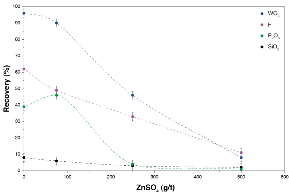
Figure 44. WO 3 , F, P 2 O 5 , and SiO 2 recoveries as a function of the ZnSO 4 dosage added prior to Na 2 SiO 3 .
