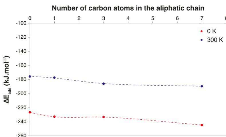
Figure 103. Evolution of the adsorption energy as a function of the aliphatic chain length at T = 0 K and T = 300 K.
