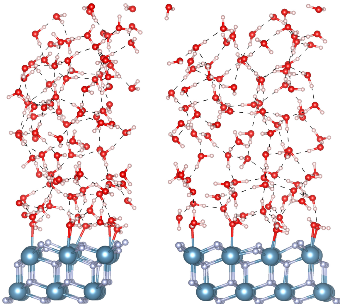
Figure 89. Snapshots of side views with 90^\circ between each other of the (111) fluorite surface with the vacuum above the surface completely filled with water molecules so that the density is 1 \text{ g.cm}^{-3} . Dashed lines represent H-bonds. The blue, grey, red, and white balls represent the calcium, fluorine, oxygen, and hydrogen atoms, respectively.
