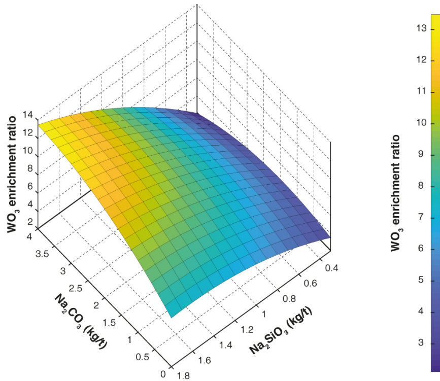
Figure 50. Response surface plot of the \text{WO}_3 enrichment ratio as a function of the \text{Na}_2\text{SiO}_3 and \text{Na}_2\text{CO}_3 concentrations.
