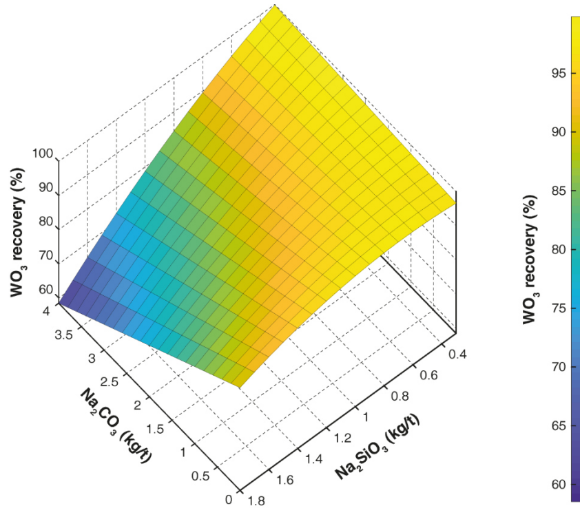
Figure 47. Response surface plot showing the \text{WO}_3 recovery as a function of the \text{Na}_2\text{SiO}_3 and \text{Na}_2\text{CO}_3 concentrations.
