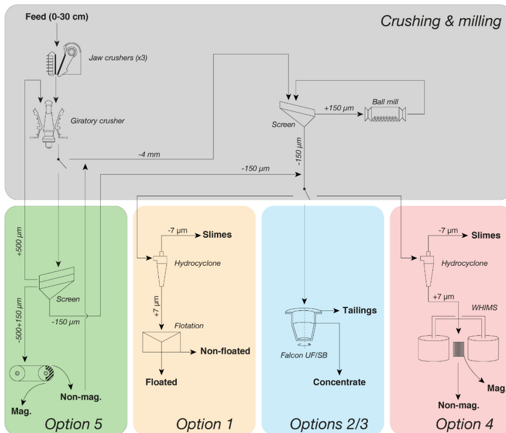
Figure 74. Global flowsheet displaying the optimised milling stage and the 5 different options investigated for processing the Main Skarn Tabuaço ore. Options 1 to 4 are performed on a milled ore (-150 \mu\text{m} ) while option 5 is performed prior to the milling stage. Options numbers correspond to the numbers introduced in the text.
