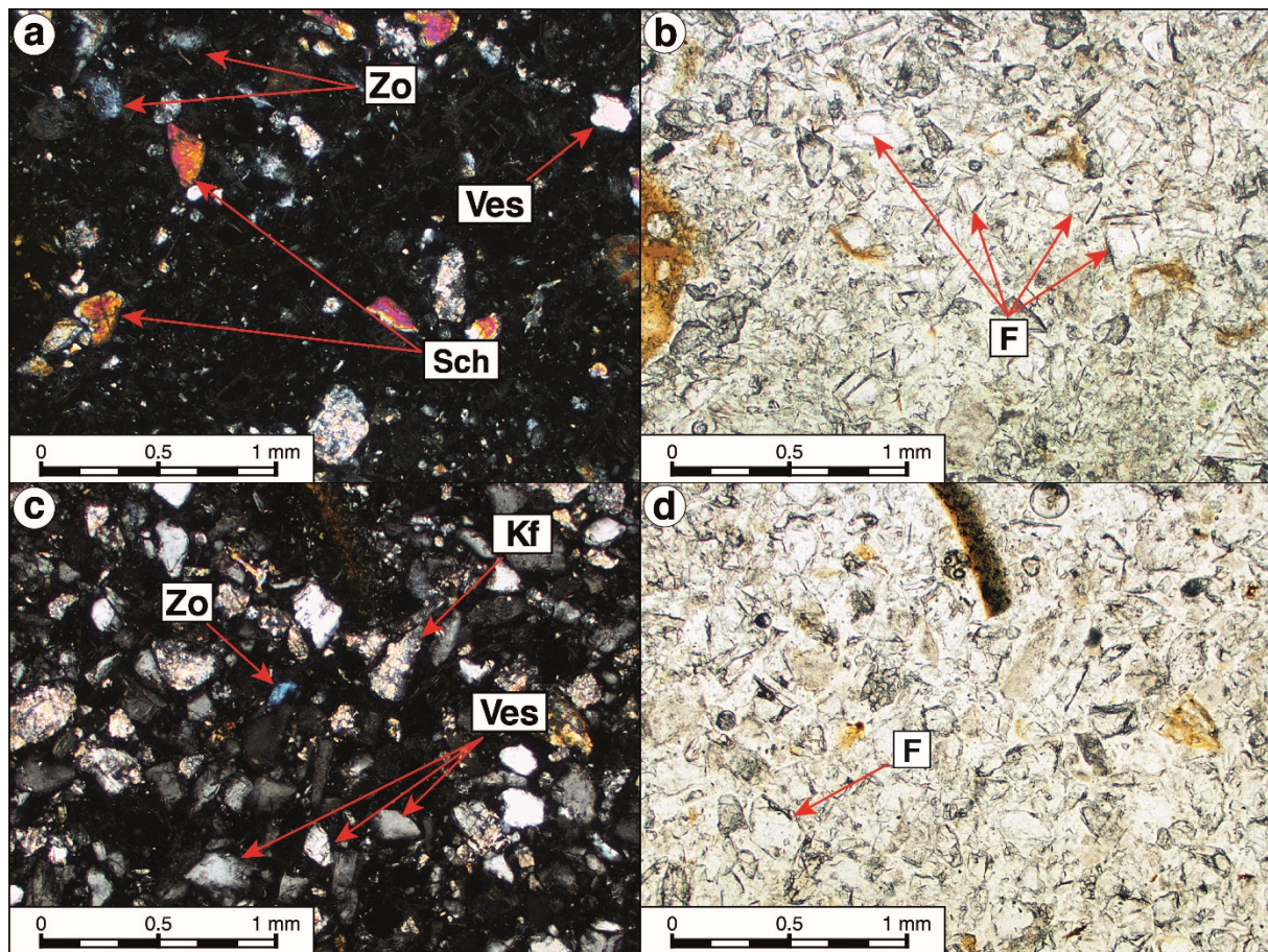
Figure 75. Micrographs of thin sections of the concentrate (a, b) and the tailings (c, d) of the flotation test with optimised depressants conditions observed with an optical microscope under cross-polarised light (a, c) and polarised light (b, d). F = Fluorite; Ves = Vesuvianite; Zo = Zoisite; Kf = K-feldspar; Sch = Scheelite.
