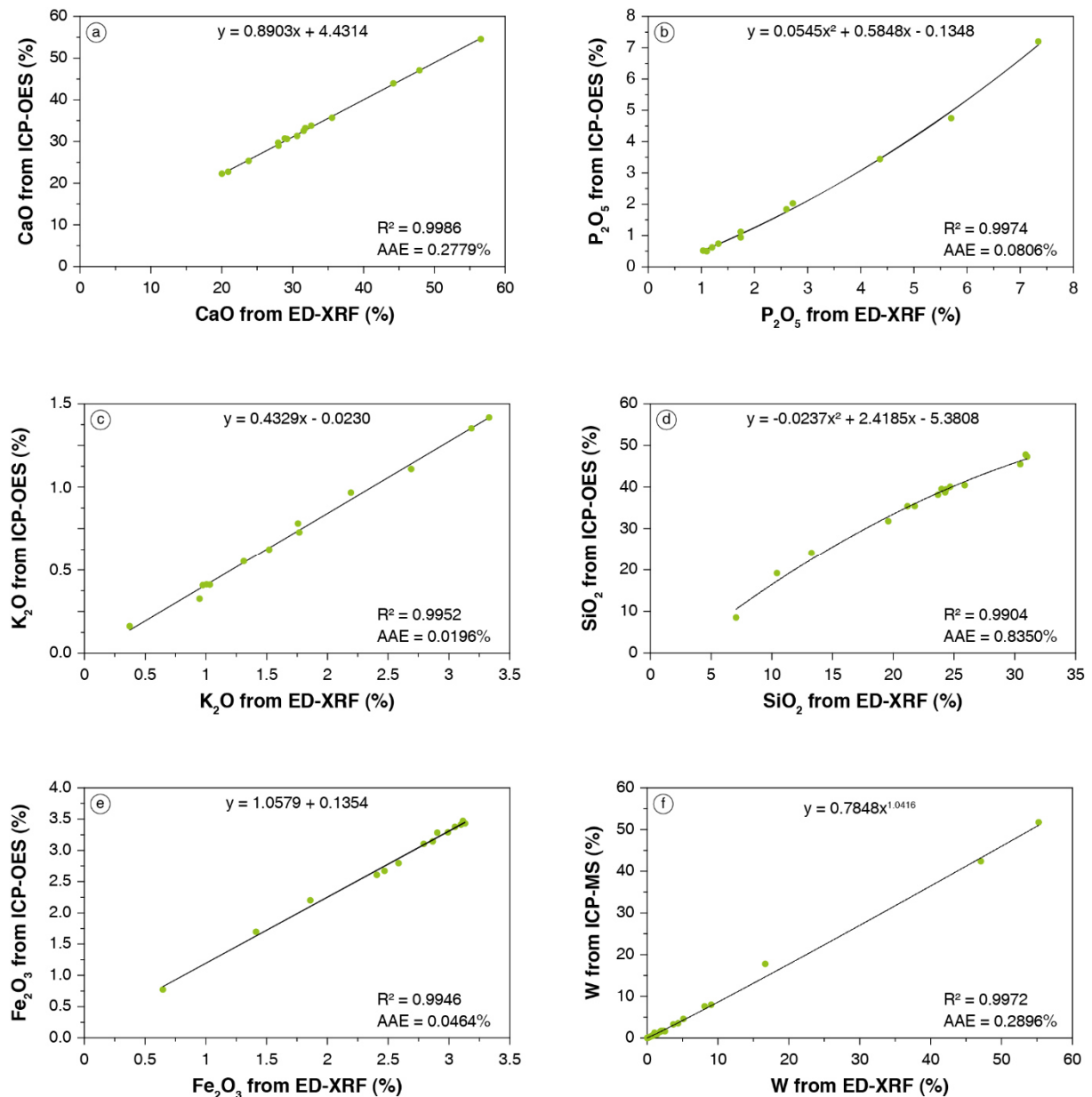
Figure 24. CaO (a), P_2O_5 (b), K_2O (c), SiO_2 (d), Fe_2O_3 (e), and W (f) contents measured by ICP-OES/MS as a function of the same contents measured by ED-XRF using a Niton™ XL3t (Thermo Scientific) portable analyser. The graphs display the model developed on the data, their squared correlation coefficient ( R^2 ), and their absolute average error (AAE). This latter value assesses the error that can be done when predicting the content with the model.
