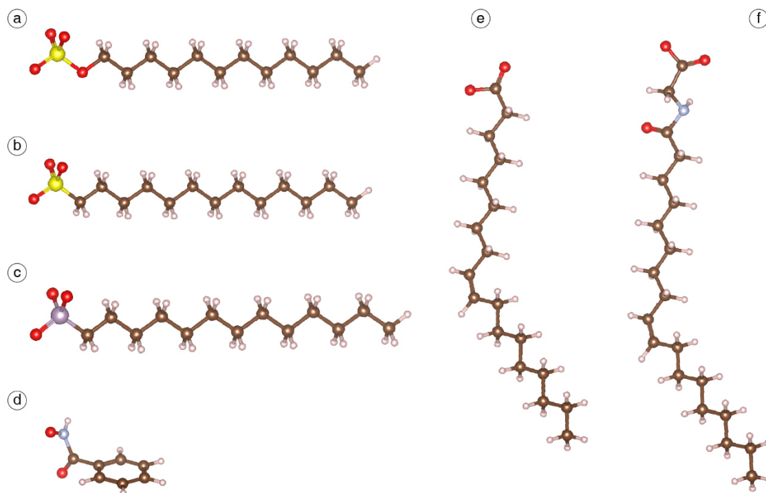
Figure 13. The different anionic collector families used for scheelite flotation: sulphates (a), sulphonates (b), phosphonates (c), hydroxamates (d), carboxylates (e), and sarcosinates (f). The marron, white, red, yellow, purple, and blue-grey balls represent the carbon, hydrogen, oxygen, sulphur, phosphorous, and nitrogen atoms, respectively.
