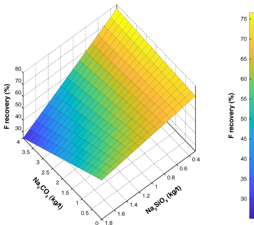
Figure 48. Response surface plot presenting the F recovery as a function of the \text{Na}_2\text{SiO}_3 and \text{Na}_2\text{CO}_3 concentrations.
