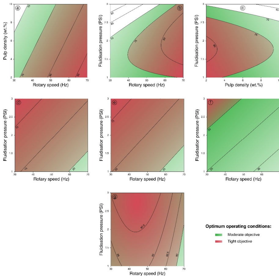
Figure 37. 2-D contour plots for WO 3 recovery (a, b, c), K 2 O recovery (d), P 2 O 5 recovery (e), Fe 2 O 3 recovery (f), and desliming efficiency (g) for the Falcon SB models as a function of the operating parameters. The green and the red zones correspond to values which satisfy respectively the moderate and the tight performance objectives defined in Table 8.
