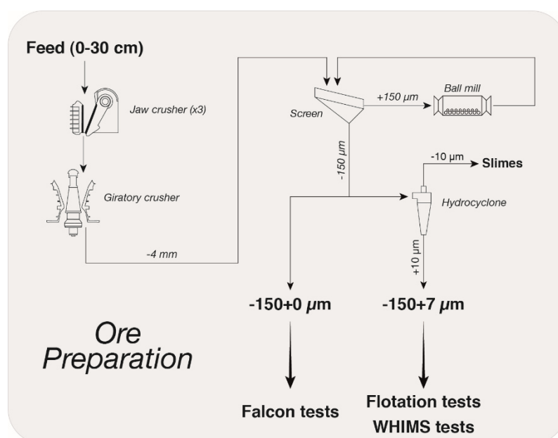
Figure 27. Schematic diagram showing the ore comminution for preparation of -150+0 \mu\text{m} and -150+7 \mu\text{m} products, used for metallurgical test work, from the Main Skarn blocs sampled in Tabuaço.
