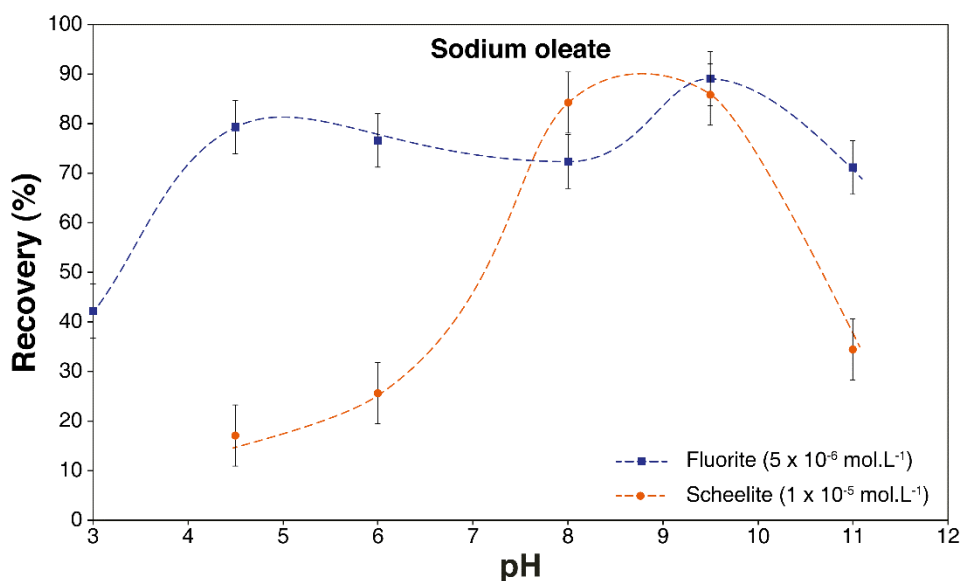
Figure 58. Microflotation recoveries of fluorite and scheelite as a function of the conditioning and flotation pH, with sodium oleate at set concentration.
