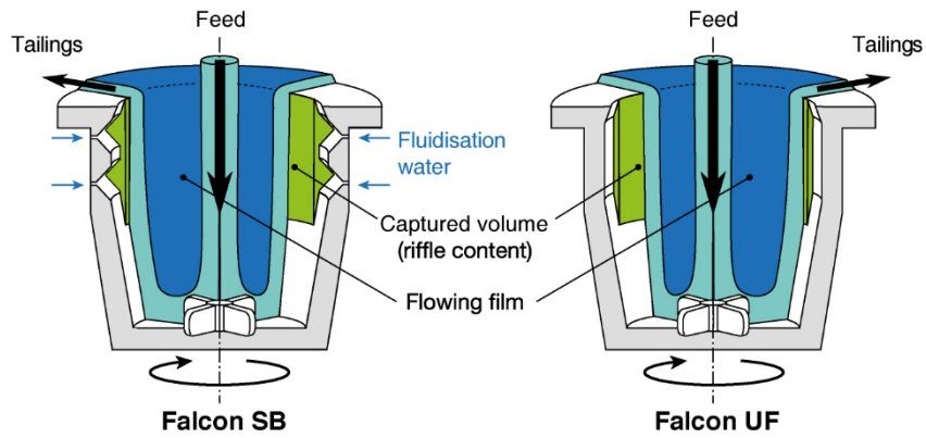
Figure 11. Falcon L40 SB (left) and UF (right) bowl schematics cross-sections, adapted from (Filippov et al., 2016; Kroll-Rabotin et al., 2010).
