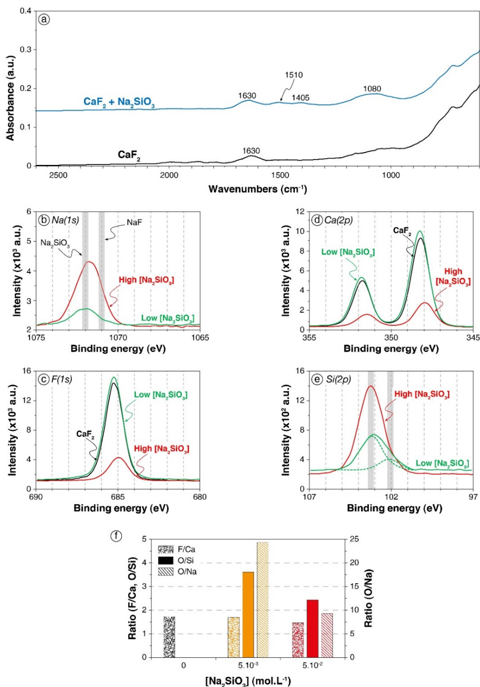
Figure 55. Adsorption of \text{Na}_2\text{SiO}_3 onto \text{CaF}_2 surface. a. Infrared spectra of \text{CaF}_2 conditioned in deionised water (black) and in a 5.10^{-2} mol.L ^{-1} \text{Na}_2\text{SiO}_3 solution (blue). b. XPS \text{Na}(1s) spectra of \text{CaF}_2 conditioned in a 5.10^{-3} mol.L ^{-1} (green) and a 5.10^{-2} mol.L ^{-1} (red) \text{Na}_2\text{SiO}_3 solutions, with the common binding energies of Na-O and Na-F bonds [from (Briggs, 1981)]. c. XPS \text{F}(1s) spectra, same legends than above. d. XPS \text{Ca}(2p) spectra, same legends than above. e. XPS \text{Si}(2p) spectra, same legends than above, with the common binding energies of \text{SiO}_2 and Si-O-X bonds (Barr, 1978; Carniato et al., 2007; Merlen et al., 1990). f. F/Ca, O/Si, and O/Na ratios of \text{CaF}_2 conditioned in deionised water (black), in a 5.10^{-3} mol.L ^{-1} \text{Na}_2\text{SiO}_3 solution (orange), and in a 5.10^{-2} mol.L ^{-1} \text{Na}_2\text{SiO}_3 solution (red). The ratios were calculated with the corresponding component for O and Si.
