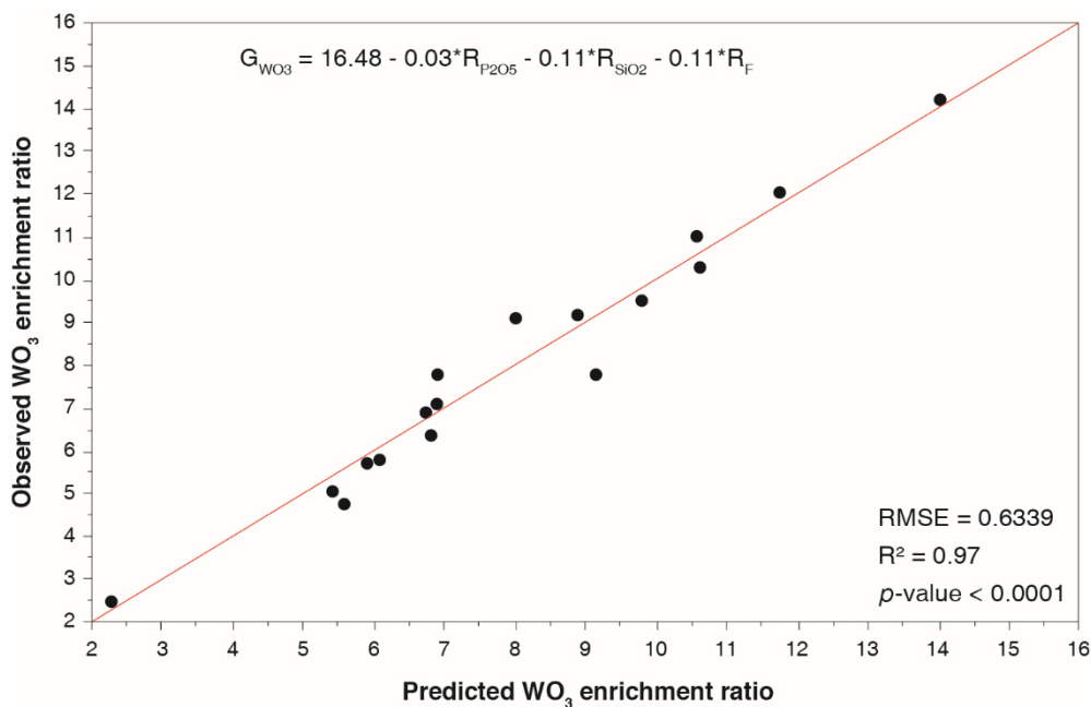
Figure 51. Observed versus predicted values for the WO 3 enrichment ratio modelled as a function of P 2 O 5 , SiO 2 , and F recoveries; the formula is included on the top of the figure.
