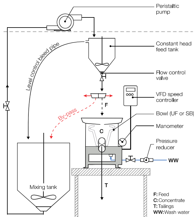
Figure 30. Experimental setup for Falcon L40 testing. Note that wash water (WW) is only used for Falcon SB testing.
