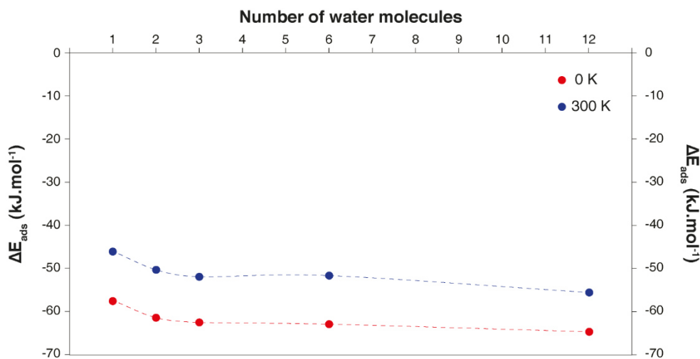
Figure 88. Internal adsorption energies calculated from the AIMD calculations for different water coverages, confirming the results obtained at 0 K.
