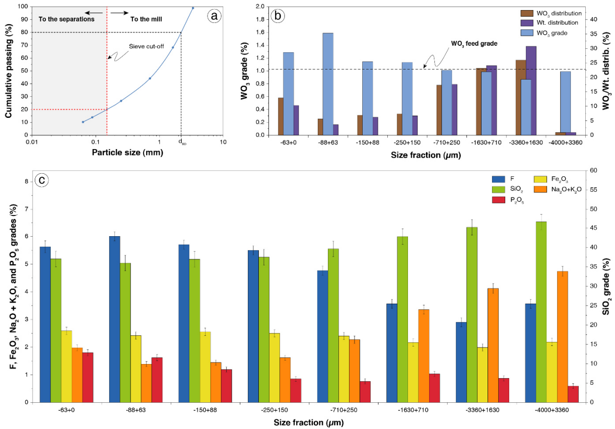
Figure 28. a. PSD of the Main Skarn Tabuaço ore after the crushing stage and before the milling stage. The size cut-off applied by the sieve before the crushing stage is displayed as well as the d_{80} of the product, corresponding to the size which 80 wt.% of the particles are finer than. b. WO_3 grade, WO_3 distribution, and wt.% retained for each size fraction of the crushed product (0-4 mm), after the gyratory crusher. Since the WO_3 grade was measured by ICP-MS, the error bars are not displayed considering the accuracy of this method. c. F, SiO_2 , Fe_2O_3 , Na_2O + K_2O , and P_2O_5 grades in each size fraction of the crushed ore, assessing the distributions of the main gangue minerals in the different size fractions. The error bars represent the average error claimed for each analysis method (ISE for F, ICP-AES for the other), which is roughly equivalent to 5% of the given value.
