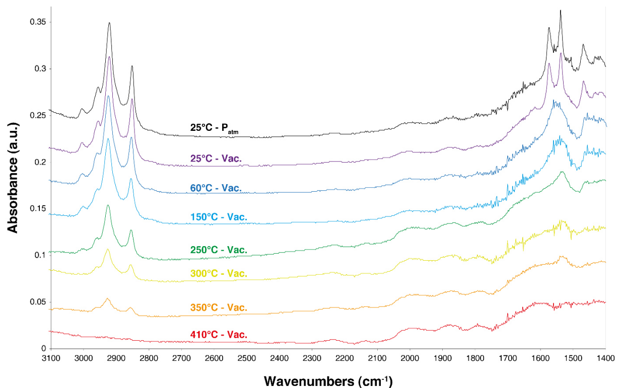
Figure 116. DRIFT spectra of a fluorite sample conditioned in a solution of sodium oleate at 1 \times 10^{-4}\text{ mol.L}^{-1} with different pressures and increasing temperatures. The IR spectrum of pure fluorite has not been subtracted here.
