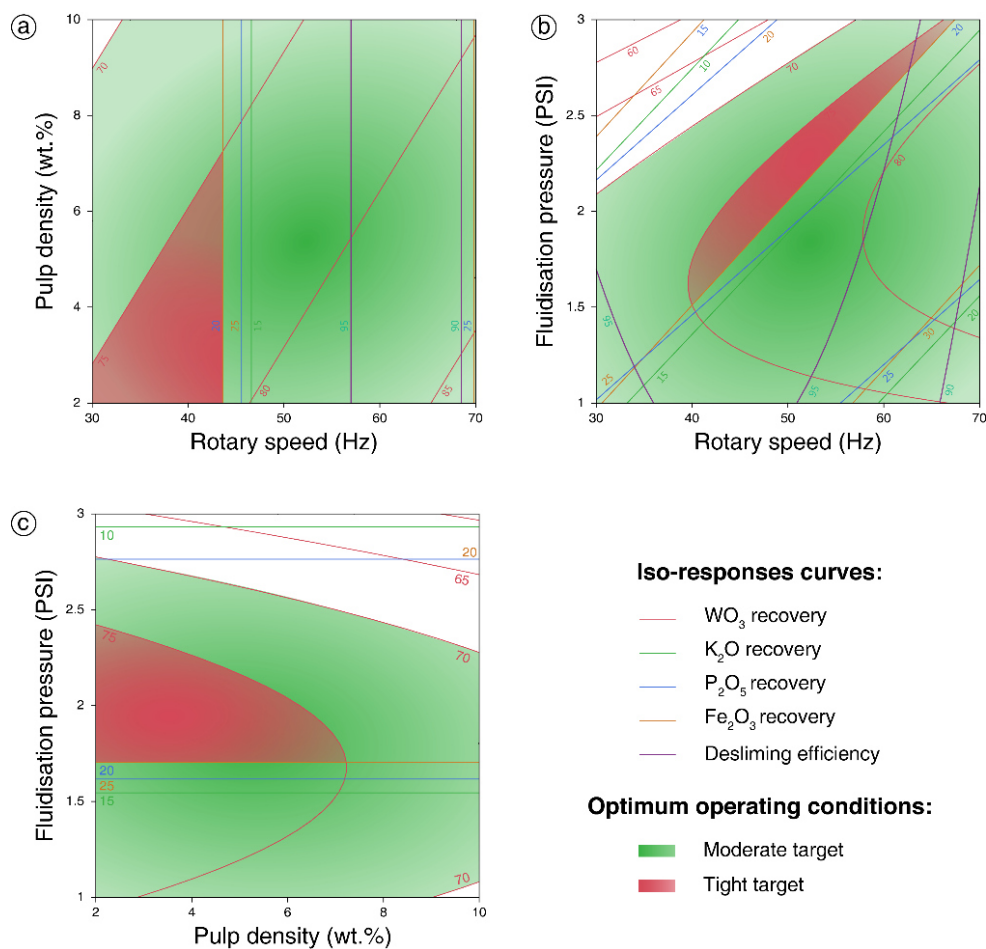
Figure 38. 2-D contour plots for the 5 studied responses ( \text{WO}_3 , \text{K}_2\text{O} , \text{Fe}_2\text{O}_3 , and \text{P}_2\text{O}_5 recoveries and desliming efficiency) for the Falcon SB models as a function of the operating parameters. Targets represent zones where the objectives set on all the studied responses, defined in Table 8, are reached.
