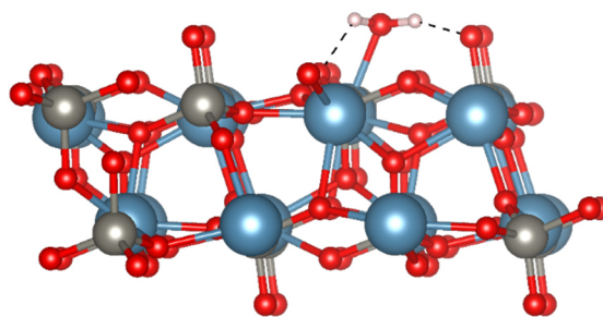
Figure 94. Adsorption of molecular water on the (112) scheelite surface. Only the upper part of the surfaces are displayed here. The blue, dark grey, red, and white balls represent the calcium, tungsten, oxygen, and hydrogen atoms, respectively.
