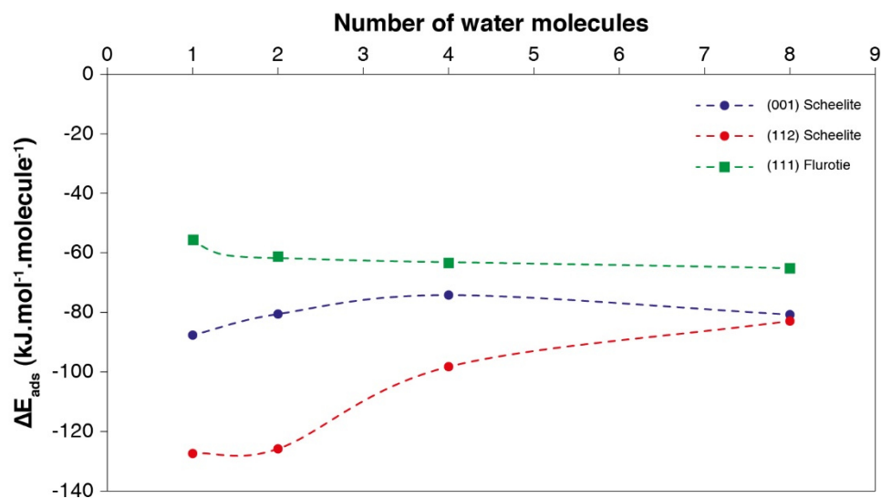
Figure 97. Comparison of the surface coverage with water molecules on the three different studies surfaces.
