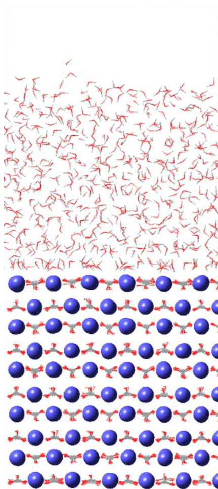
Figure 21. Snapshot of MD simulations using force fields to investigate the hydration mechanisms of calcite surface, adapted from (Perry et al., 2007).
