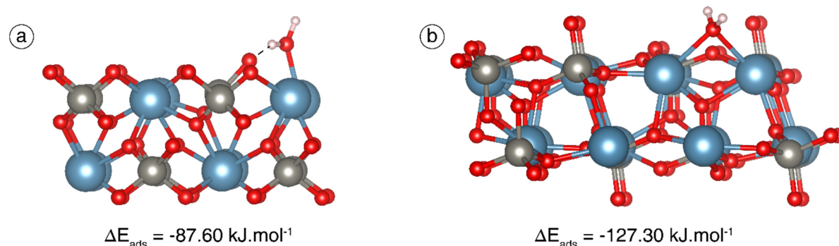
Figure 92. Adsorption of dissociated water molecule with short OH-H distance onto (001) (a) and (112) (b) scheelite surfaces. Only the upper part of the surfaces are displayed here. The blue, dark grey, red, and white balls represent the calcium, tungsten, oxygen, and hydrogen atoms, respectively.
