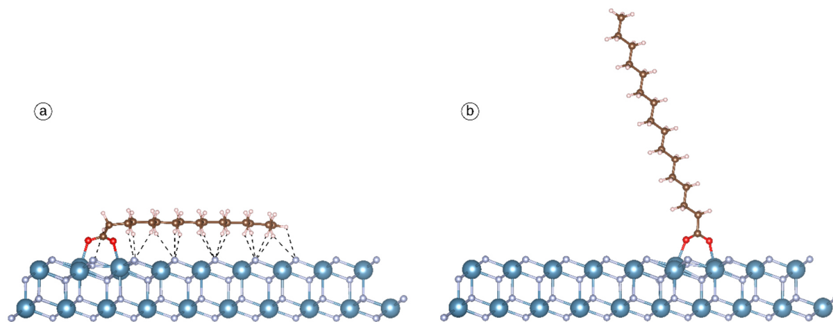
Figure 102. Adsorption of a hexadecanoate (palmitate) molecule (15 carbon atoms in the chain) in “flat” adsorption (a) and in “vertical” adsorption (b) after DFT relaxation. The blue, grey, red, marron, and white balls represent the calcium, fluorine, oxygen, carbon, and hydrogen atoms, respectively.
