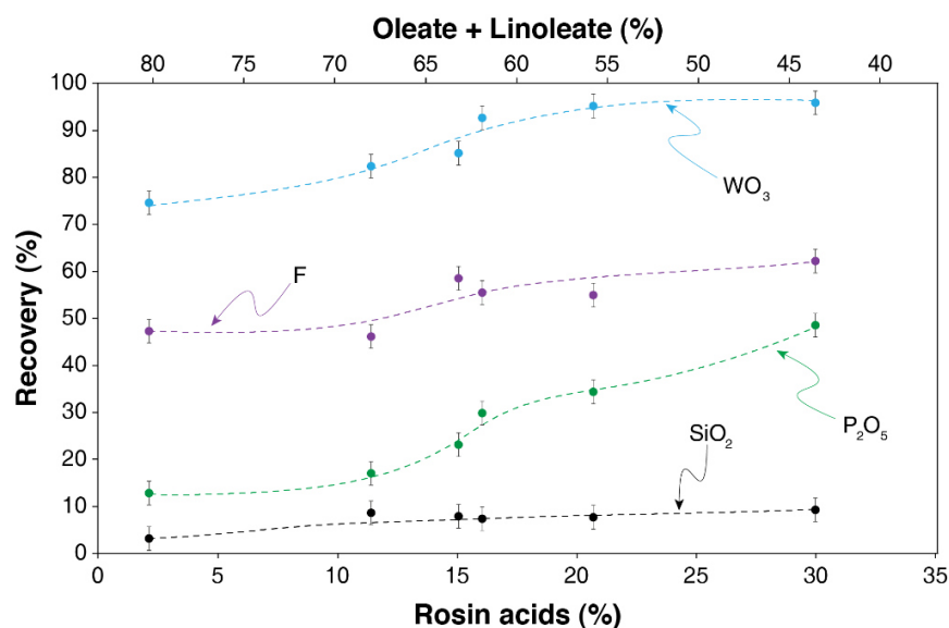
Figure 67. F, P 2 O 5 , SiO 2 , and WO 3 recoveries versus the rosin acids content in the collector mixture.
