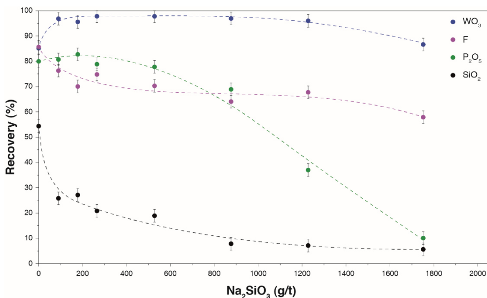
Figure 41. WO 3 , F, P 2 O 5 , and SiO 2 recoveries as a function of Na 2 SiO 3 dosage.
