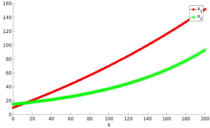
Figure C.1: State evolution for OP_{\min, \text{stop}} with \varepsilon = 5 and x = (10, 15) .
