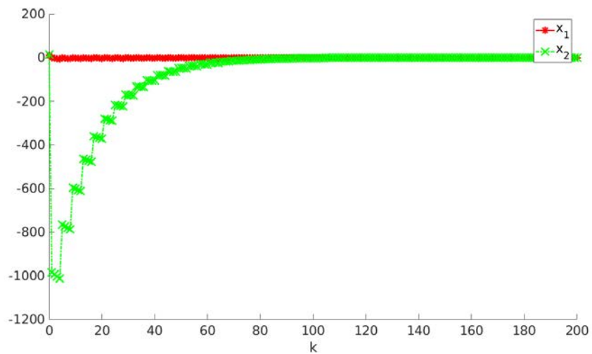
Figure C.4: State evolution for OP_{\min, \text{stop}} with \varepsilon = \frac{10}{12} = 0.833 and x = (10, 15) .
