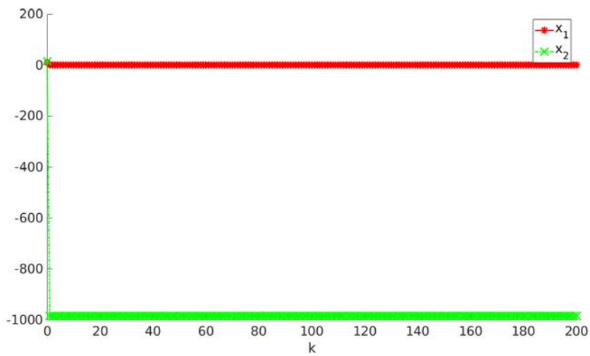
Figure C.2: State evolution for OP_{\min, \text{stop}} with \varepsilon = \frac{10}{9} = 1.111 and x = (10, 15) .
