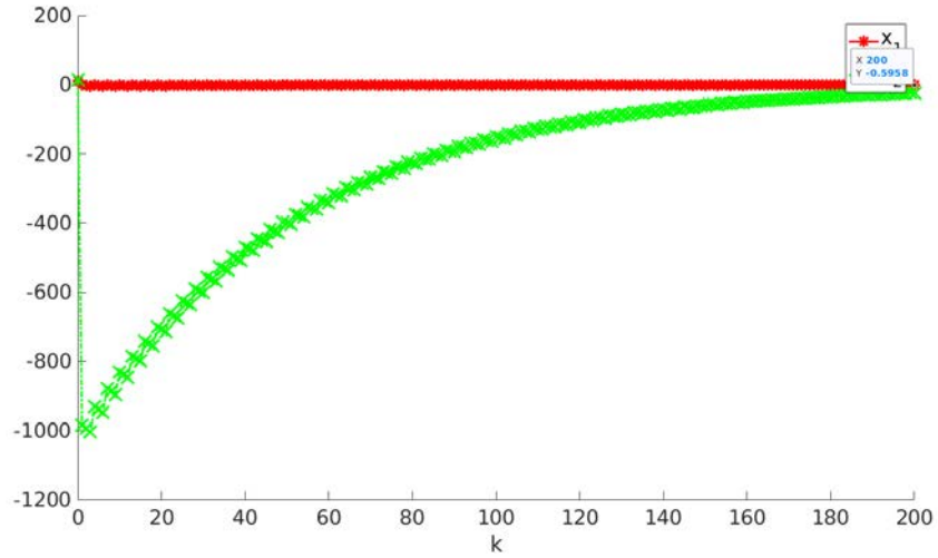
Figure C.3: State evolution for OP_{\min, \text{stop}} with \varepsilon = \frac{10}{11} = 0.909 and x = (10, 15) .
