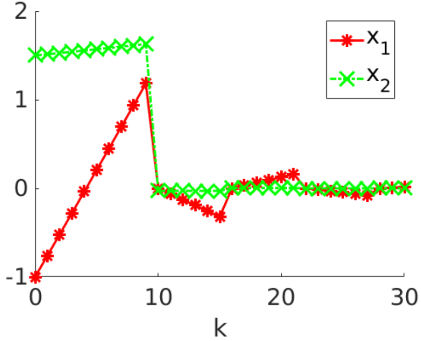
Figure 3.1: State evolution for OP_{\min,budget} with B = 3000 and x = (-1, 1.5) .
