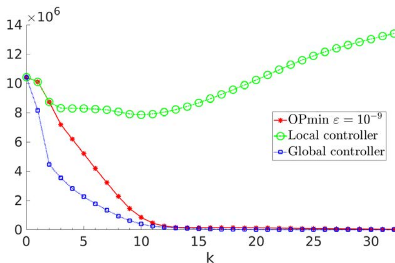
Figure 3.2: \sigma(\phi(\cdot, x)) for inputs given by OP_{\min, \text{stop}} , g(1, x) and g(2, x) .
