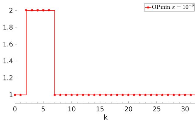
Figure 3.3: Input selection of OP_{\min, \text{stop}} for x_0 = (10, -10, -10, -10) .
