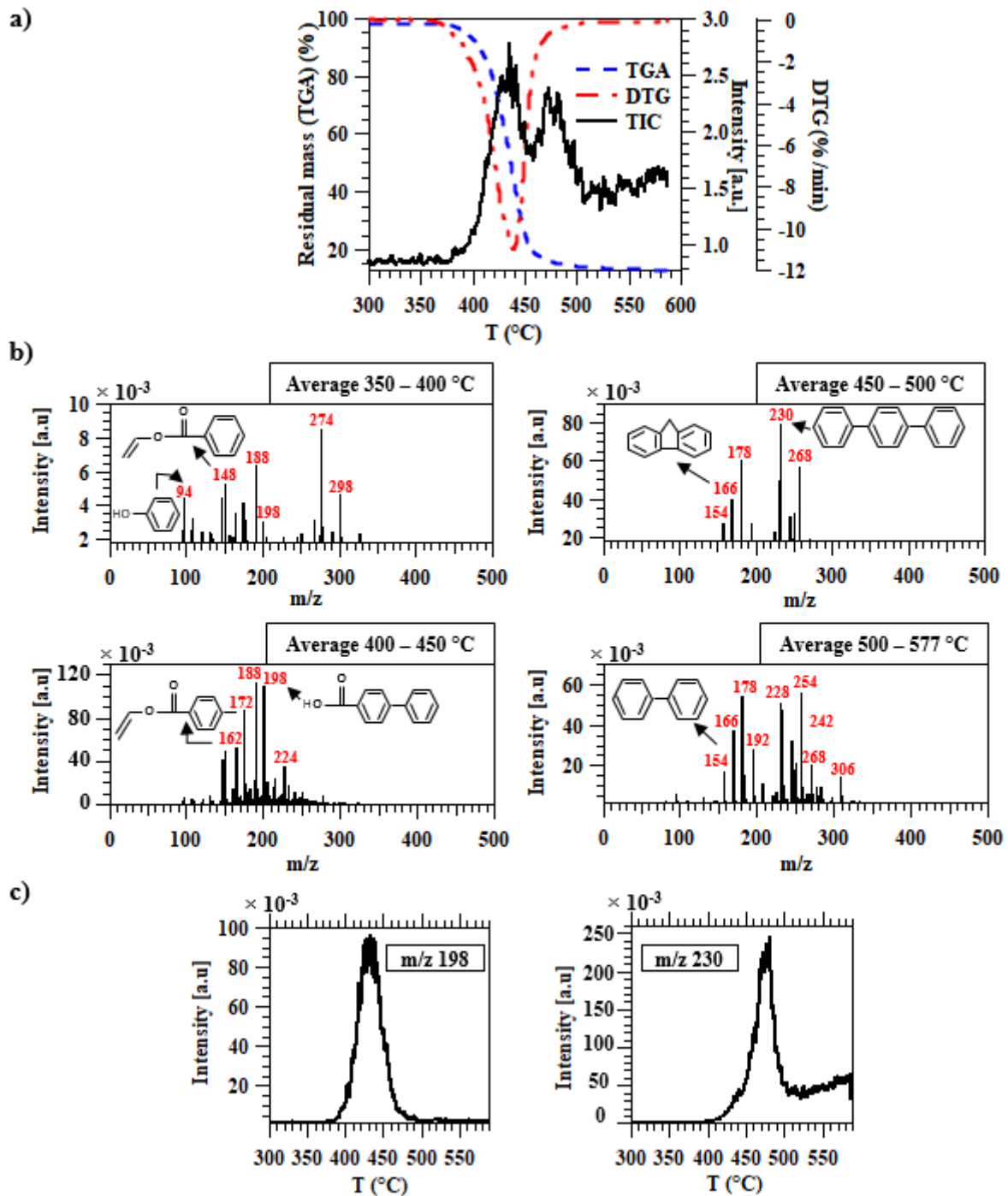
Figure V. 4: TGA-REMPI TOF-MS results: a) TGA, DTG, TIC curves, b) Average mass spectra of the products at various temperatures, c) thermal evolution profiles of major m/z .
