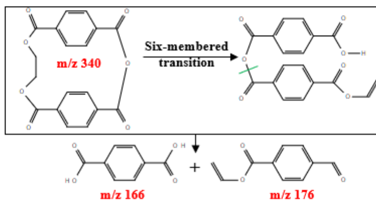
Figure V. 9: Proposed reaction pathways for the degradation of: a/cyclic dimer, b/ cyclic anhydride.
