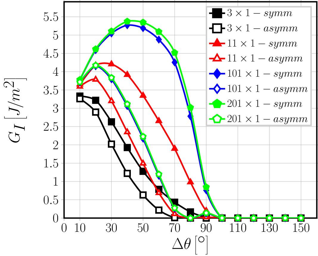
Figure 5: Comparison of Mode I ERR between n \times 1 – symm and n \times 1 – asyymm RVEs, V_f = 60\% , \varepsilon_x = 1\% .
