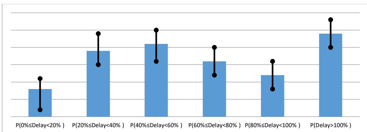
Figure 4.11. Precision (black line) for the six states in a target node
