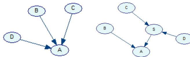
4.6a. Without synthetic node, the model needs 256 values.
