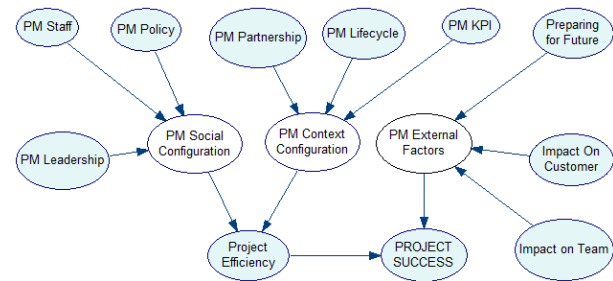
Figure 4.12-b. Proposed BN with synthetic nodes.
