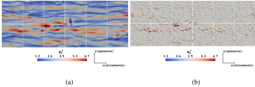
Figure 3.17 – Instantaneous velocity field in the plane z^+ = 4 from DNS without turbulence forcing as (a) color map of its streamwise component and (b) vector field.
