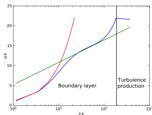
Figure 3.12 – Mean velocity profiles for the DNS simulation (blue) and comparison with traditional law of wall, u^+ = z^+ represents viscous sublayer (red line), u^+ = 2.44 \ln y^+ + 5.5 represents log-law turbulent profile.
