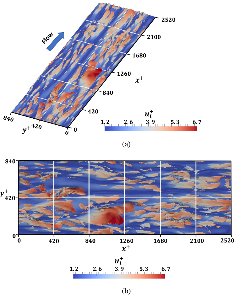
Figure 3.30 – Isocontour of q from equation (3.21) colored by instantaneous streamwise velocity component in the viscous sublayer region at turbulence intensity \gtrsim 10\% : (a) 3D view and (b) top view, q^+ = 0.00085 .
