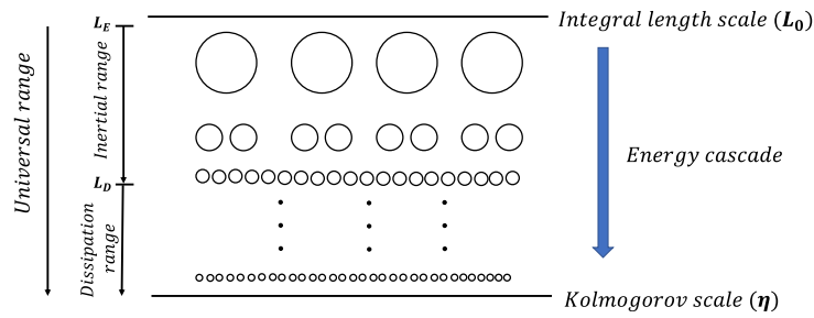
Figure 2.4 – Energy cascading in turbulent flows
