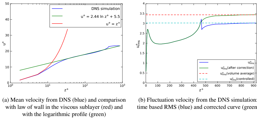
Figure 3.27 – Velocity profiles along the wall-normal direction from simulation performed at \approx 10\% turbulent intensity.
