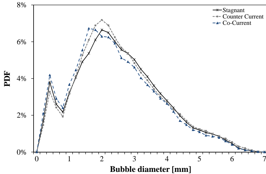
Figure 4.34 – Equivalent diameter distribution measured at the 5 elements outlet. Q_G = 2.5 l/h, d_n = 0.2 mm.
