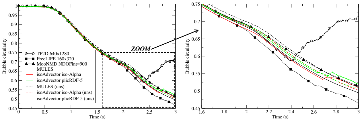
Figure 6.9 – Bubble circularity at resolution 640 \times 1280 . Comparison of MULES, isoAdvect isoAlpha and plicRDF-5 with reference data for both Cartesian and triangular grids.
