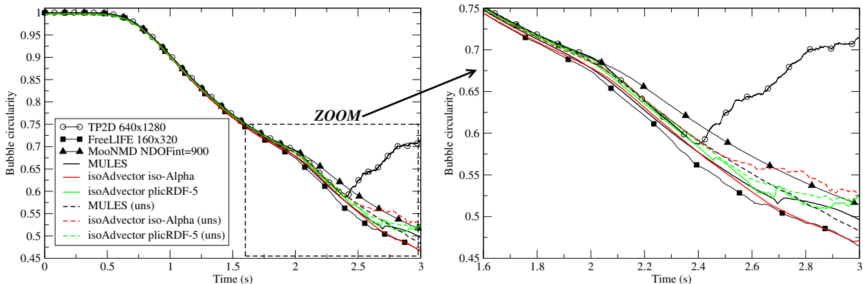
Figure 6.8 – Bubble circularity at resolution 160 \times 320 . Comparison of MULES, isoAdvect isoAlpha and plicRDF-5 with reference data for both Cartesian and triangular grids.
