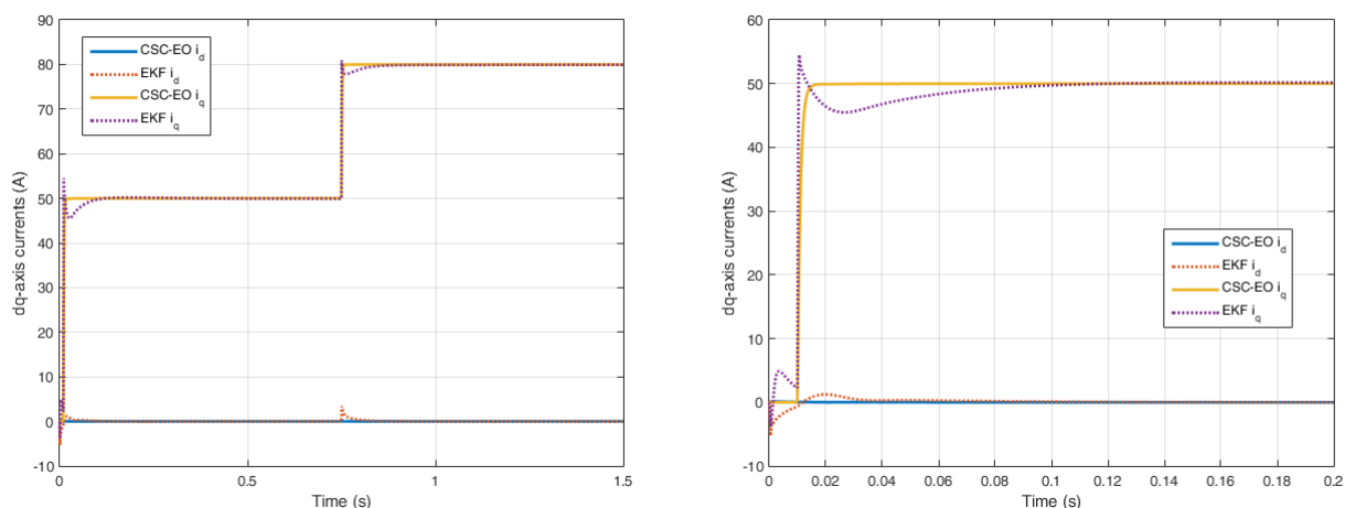
Figure 3.22. Performance comparison between the CSC-EO and the EKF + PI solution with no parameter error
