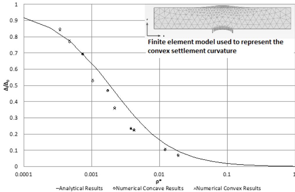
Fig. V.13: Results of the numerical comparison between concave and convex soil curvatures for the deflection transmission ratio.
