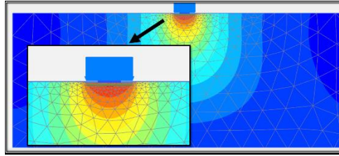
Fig. XIII.3. Beam and soil displacements.
