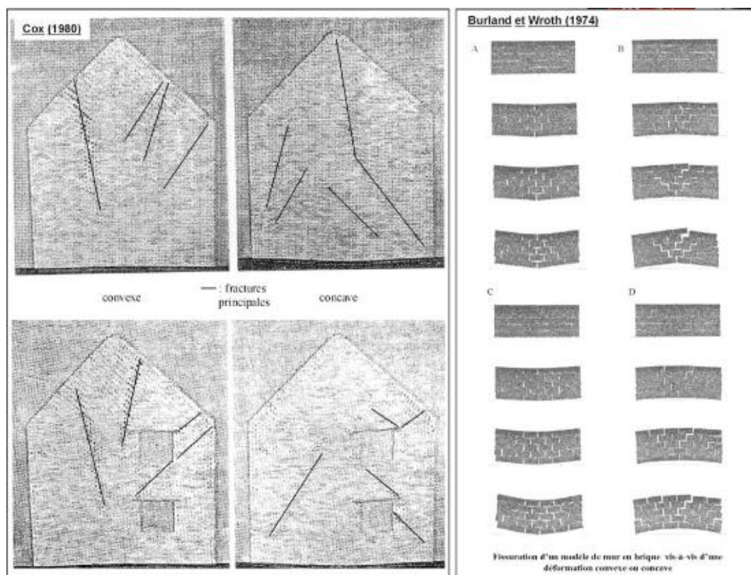
Fig. II.8 Experiments highlighting the behavior of a masonry structure and the orientation of cracking - Deck (2002)
