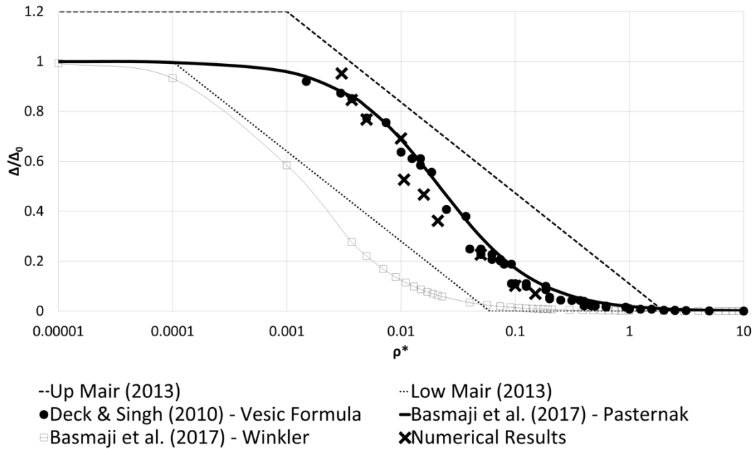
Fig. VI.10. Comparison between Mair (2013); Deck & Singh (2010); Pasternak-Basmaji et al. (2017); Winkler-Basmaji et al. (2017) and numerical results.
