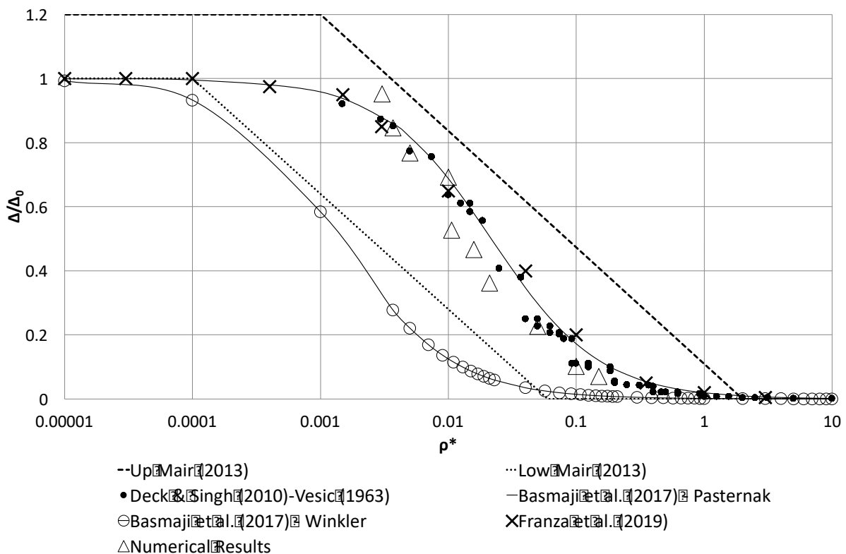
Fig. IV.4. Comparison between Mair (2013); Deck & Singh (2010); Pasternak-Basmaji et al. (2017); Winkler-Basmaji et al. (2017), Franza et al. (2019) results and numerical (Plaxis 2D) results.
