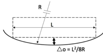
Fig. IV.2 Free-field deflection \Delta_0 .
