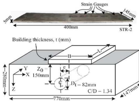
Fig. II.31 Building representation by the physical model (Farrell et al. (2014) [58]).
