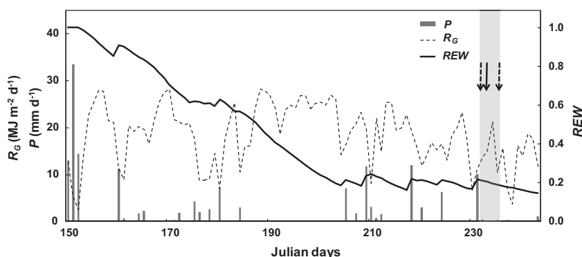
Fig. 2. Seasonal pattern of modelled daily relative soil extractable water (REW, solid line), daily sum of precipitation ( P , mm\ d^{-1} , grey bars) and daily sum of global radiation ( R_G , MJ\ m^{-2}\ d^{-1} , dashed line) during the summer 2013 (Julian days 150–243). The period indicated in grey represents the duration of the experiment. The vertical bold arrow represents the date of isotope labelling. The vertical dashed arrows represent the date of soil and branch sampling one day before and three days after labelling.
