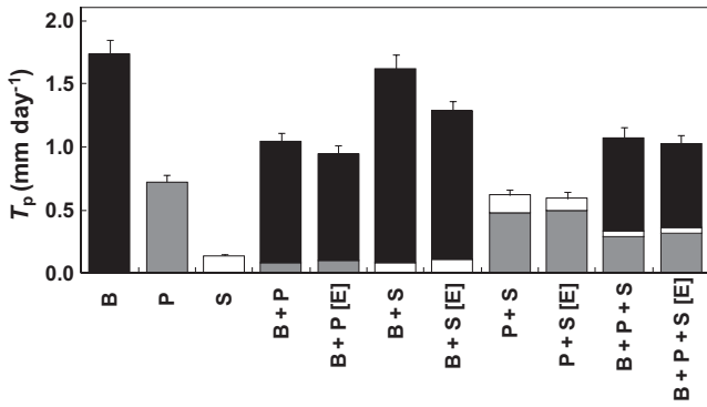
Fig. 5. Mean observed and expected ([E]) plot transpiration ( T_p ; mm day -1 ) in monocultures and mixtures of birch (B), pine (P) and spruce (S) during the two measurement periods (7–12 July, 2011 and 2–8 August, 2011). Vertical bars are standard errors of the mean for the 13 days of sap flux density measurements.
