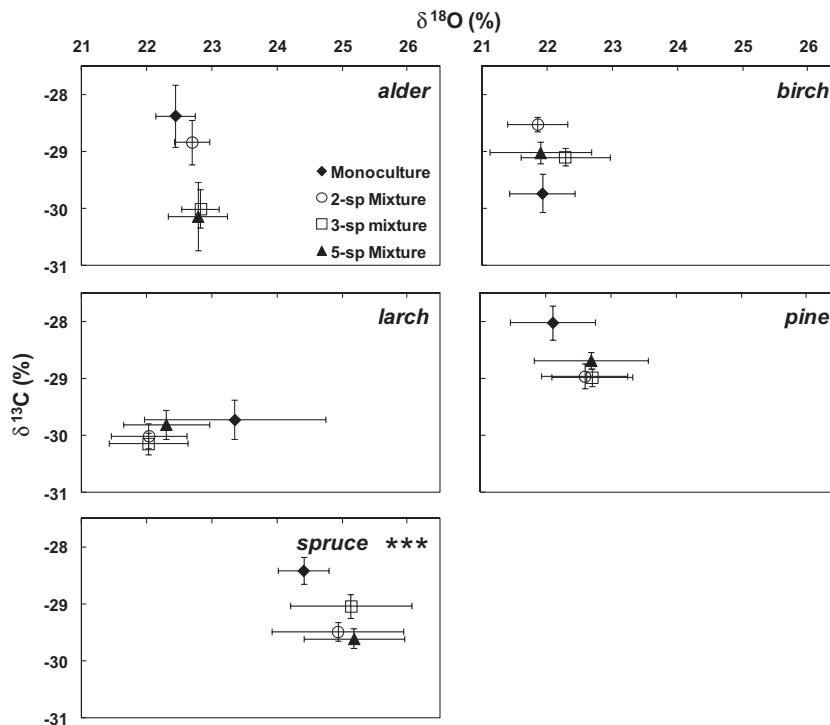
Fig. 6. Relationship between mean leaf or needle carbon and oxygen isotope composition ( \delta^{13}C and \delta^{18}O , ‰) for alder, birch, larch, pine and spruce in monocultures, two-species mixtures, three-species mixtures and five-species mixtures. Bars are standard errors of the mean for 10 sampled trees. Asterisks denote significant linear relationships between \delta^{13}C and \delta^{18}O (type II regression; *** P < 0.001 ).
