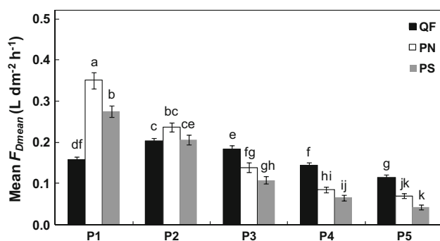
Fig. 3 Mean of the daily mean sap flux density (Mean F_{Dmean} , L dm -2 h -1 ) for Quercus faginea (QF), Pinus nigra (PN) and Pinus sylvestris (PS) for each period of measurements (P1, P2, P3, P4 and P5). Vertical bars represent the standard error of the mean for each period of measurement. Letters denote significant differences in daily mean sap flux density among all species and periods
