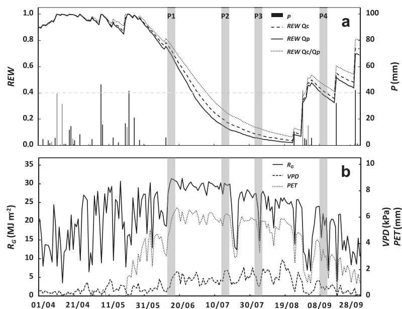
Fig. 1. Seasonal pattern of (a) modelled relative soil extractable water ( REW ) for each plot, daily sum of precipitation ( P , mm), (b) daily sum of global radiation ( R_G , \text{MJ m}^{-2} ), daily evapotranspiration ( PET , mm) and daily mean vapor pressure deficit ( VPD , kPa) during the summer 2012 (01/04/2012 to 31/09/2012). Periods indicated in grey represent the periods of sap flux density measurements (P1, P2, P3 and P4). The dashed grey line stand for the threshold of 0.4 of REW under which the resulting soil water shortage induces a drop in stomatal conductance and thus in leaf gas exchange.
