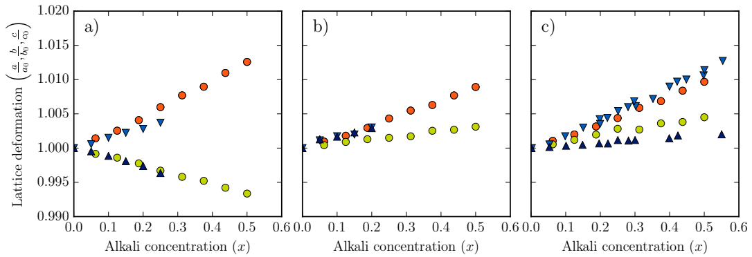
Figure 3.7 Comparison between the calculated and experimental (Kusumoto et al. , 2019; Rong-Tie et al. , 2017; Maeda et al. , 2017) lattice deformations, \frac{a}{a_0} ( \bullet ), \frac{b}{b_0} ( \circ ) and \frac{c}{c_0} ( \bullet ) of a) \text{Cu}_{1-x}\text{Li}_x\text{GaS}_2 , b) \text{Cu}_{1-x}\text{Li}_x\text{InS}_2 and c) \text{Cu}_{1-x}\text{Li}_x\text{InSe}_2 . The experimental \frac{a}{a_0} and \frac{c}{c_0} are represented by \blacktriangledown and by \blacktriangle , respectively.
