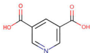
Figure I-17: Acide 3,5-Pyridinedicarboxylique
