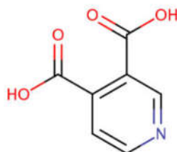
Figure I-16: Acide 2,3-Pyridinedicarboxylique
