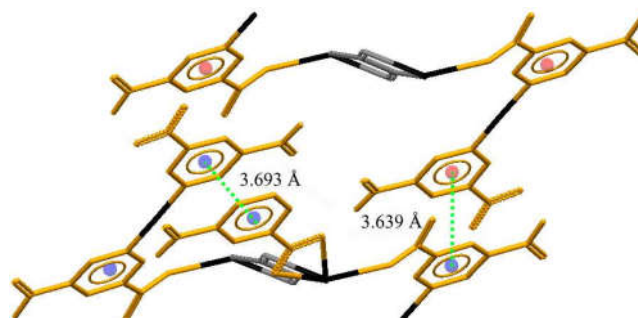
Figure 7: \pi - \pi^* stacking interactions of dinicotinate aromatic rings (all water molecules were hidden for clarity)
