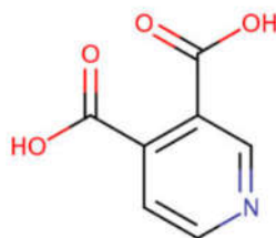
Figure I-16: Acide 2,3-Pyridinedicarboxylique
