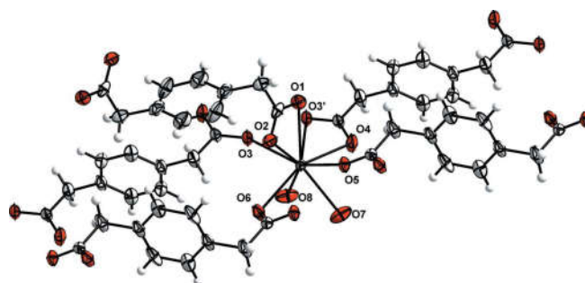
Figure 2 Coordination environment of \text{La}^{3+} in [\text{La}_2(p\text{-pda})_3(\text{H}_2\text{O})_4 \cdot 8\text{H}_2\text{O}]_\infty . Symmetry code: ( ' ) 2 - x, 1 - y, 1 - z . Hydrogen atoms of the water molecules have been omitted for clarity.
