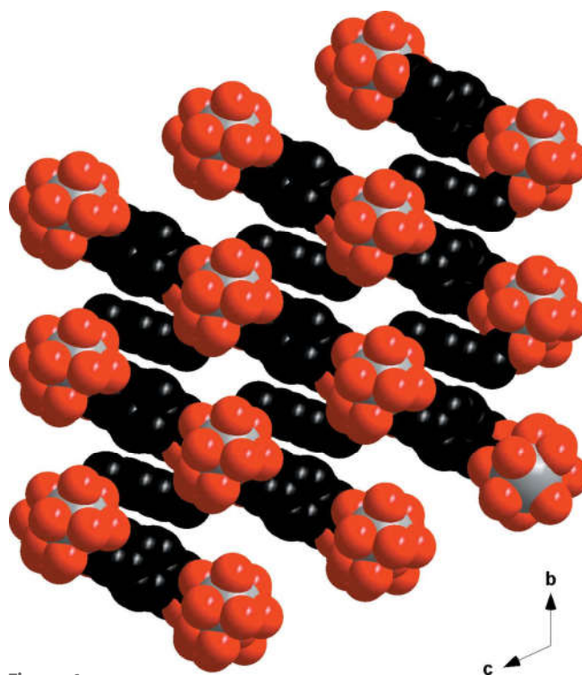
Figure 6 Projection view along the a axis of the molecular skeleton of [\text{La}_2(p\text{-pda})_3(\text{H}_2\text{O})_4 \cdot 8\text{H}_2\text{O}]_\infty in space-filling mode. Hydrogen atoms and crystallization water molecules have been omitted.
