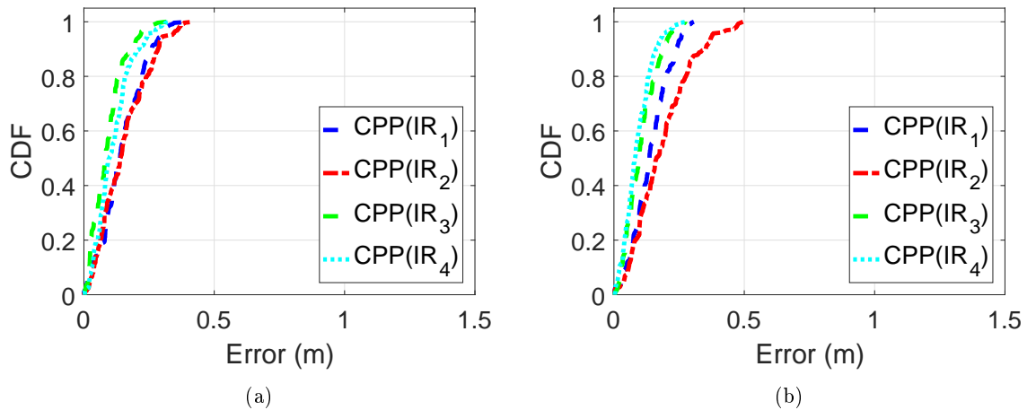
Figure 6.14: CPP performance using an imaging receiver for (a) \Delta h_{ji} = 2 m and (b) \Delta h_{ji} = 1.5 m
