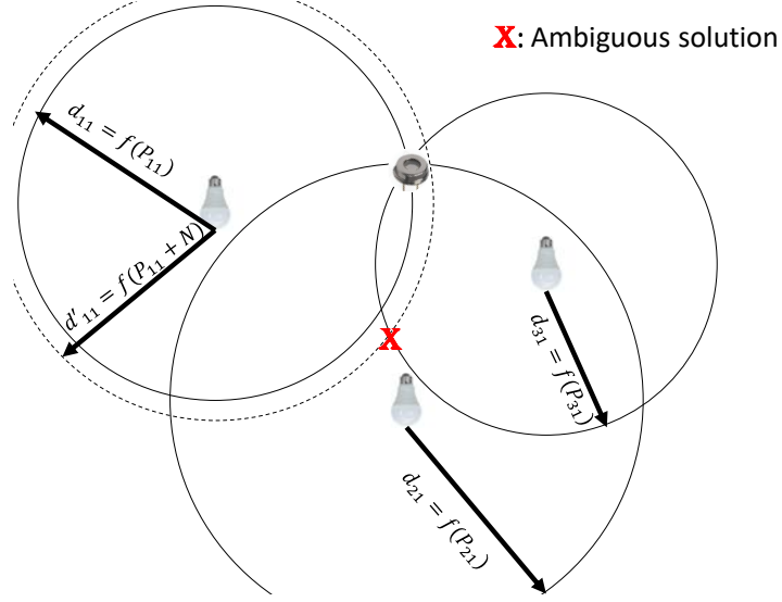
Figure 4.6: Lateration method in two dimensions based on RSS ranging
