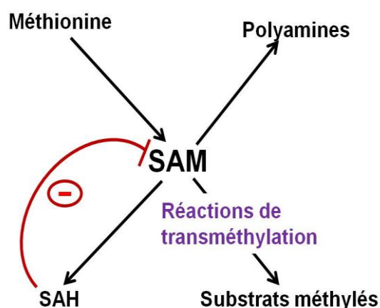
Figure 12: Inhibition of methylation reactions by SAH
