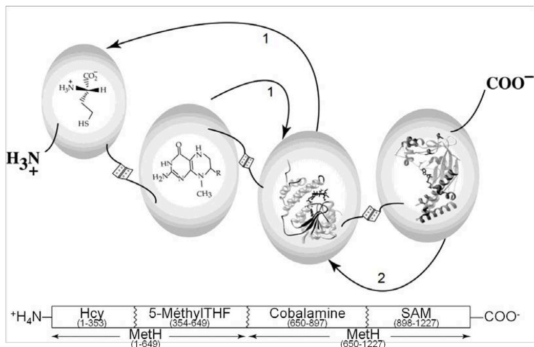
Figure 16: Diagram showing the modular structure of cobalamin-dependent methionine synthase (Rowena G Matthews, 2001)
