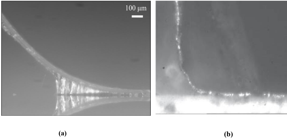
Figure 2.2: (a) Process zone for an elastic adhesive bonded on a rigid substrate for a peel test at 70^\circ [21]. The film thickness is 50 \mu\text{m} (b) Process zone of copper film bonded on a rigid substrate. The film thickness is less than 10 \mu\text{m} [22].
