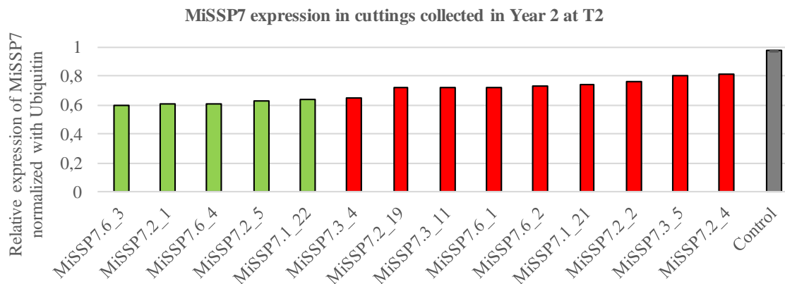
Figure 38 - The relative expression of MiSSP7 in each cutting used in this study. Relative expression of MiSSP7 normalized with Ubiquitin expression in the leaves of Populus -expressing MiSSP7 collected at T2 in Year 1 (a) and in the roots of Populus -expressing MiSSP7 collected at T1 and T2 in Year 2 (b). The green bars correspond to the cuttings with a low expression of MiSSP7 (between 0.40 and 0.60 in Year 1 and between 0.60 and 0.64 in Year 2) while the red bars correspond to the cuttings with a high expression of MiSSP7 (between 0.70 and 0.90 in Year 1 and between 0.65 and 0.80 in Year 2). The dark-grey bars correspond to the relative expression of MiSSP7 normalized with Ubiquitin in 2 weeks old ectomycorrhizae of Laccaria bicolor in Populus tremula x alba roots cultivated in axenic conditions (Control).
