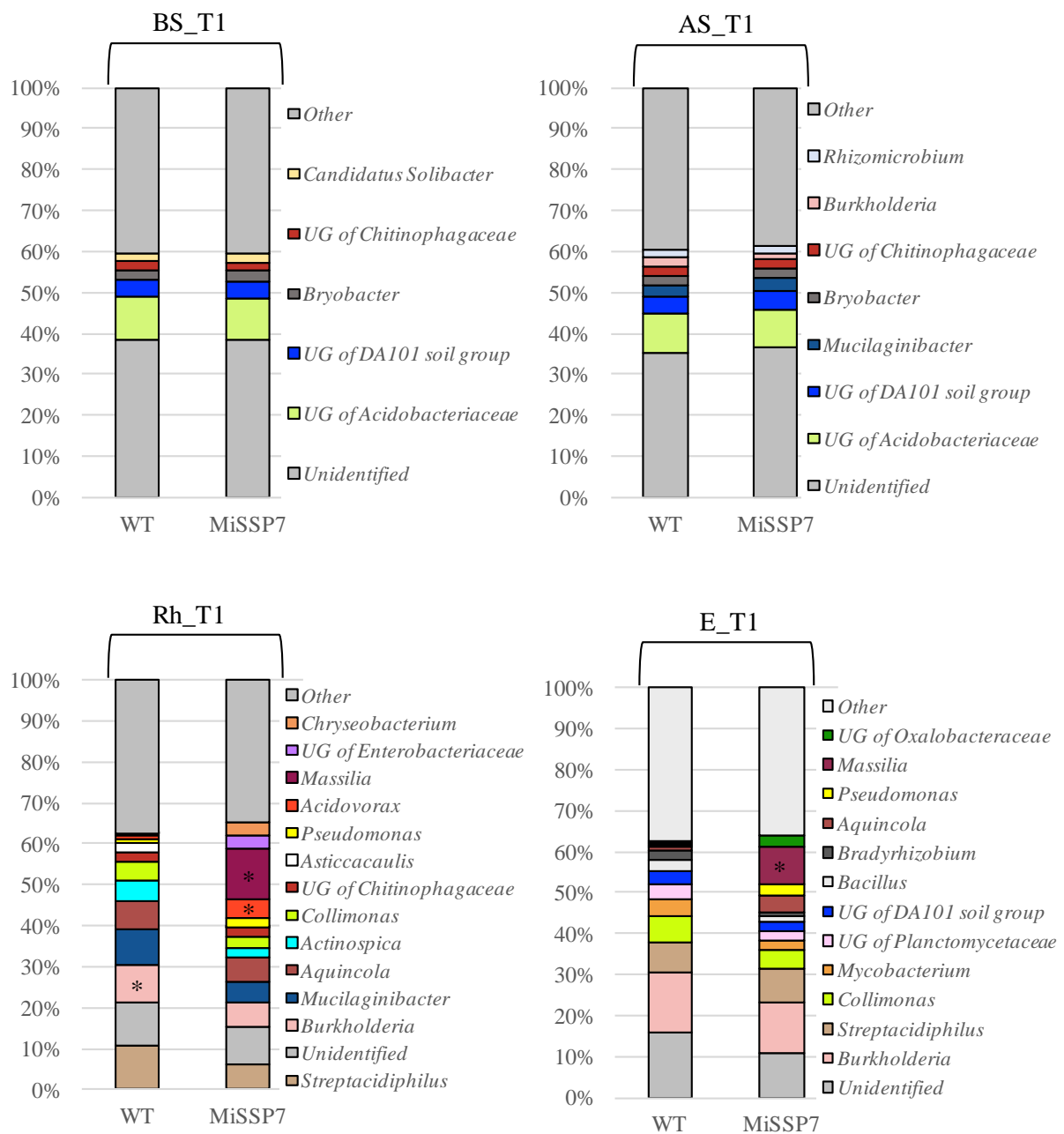
Figure S2 - The distribution of the most dominant bacterial genera (>2% in relative abundance) detected in BS, AS, Rh and E samples of Populus -expressing MiSSP7 and Populus WT cuttings collected at T1 in Year 1. The asterisks (*) denote significant difference in the relative abundance of bacterial genera detected between Populus WT and Populus -expressing MiSSP7 ( P < 0.05 , ANOVA). Detailed information is available in Table S3.
