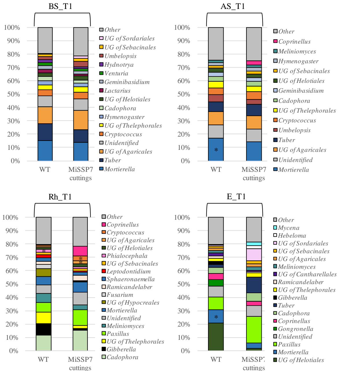
Figure S1 - The distribution of the most dominant fungal genera (>2% in relative abundance) detected in BS, AS, Rh and E samples of Populus -expressing MiSSP7 and Populus WT cuttings collected at T1 in Year 1. The asterisks (*) denote significant difference in the relative abundance of fungal genera detected between Populus WT and Populus -expressing MiSSP7 ( P < 0.05 , ANOVA). Detailed information is available in Table S2.
