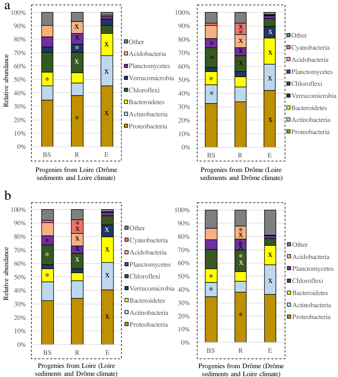
Figure 35 - Rhizosphere and root filtering effects in the non-native conditions of culture. Distribution of most dominant bacterial phyla (> 2% in relative abundance) detected in the bulk soil (BS) and in the rhizosphere (R) and the endosphere (E) of Populus nigra seedlings of the Loire and the Drôme cultivated in the non-native sediments (i.e., LDL and DLD treatments) (a) and in the non-native climate (i.e., LLD and DDL treatments) (b). The asterisks denote significant difference in relative abundance of bacterial phyla between BS and R compartments (ANOVA, P < 0.05 ). The crosses denote significant difference in relative abundance of bacterial phyla between R and E compartments (ANOVA, P < 0.05 ).
