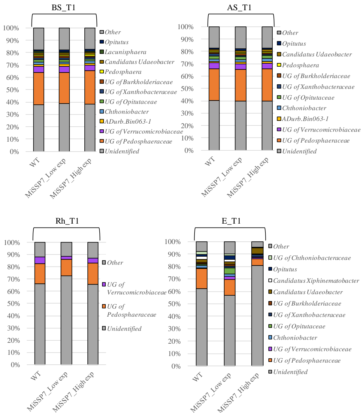
Figure S4 - The distribution of the most dominant bacterial genera (>2 % in relative abundance) detected in BS, AS, Rh and E samples of Populus -expressing MiSSP7 and Populus WT cuttings collected at T1 in Year 2. Detailed informations are available in Table S7.
