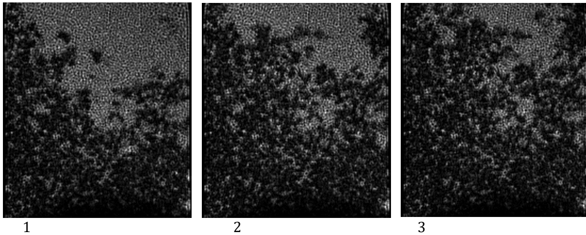
Figure 5.26. Consecutive images of the oil displaced by water in the model of polystyrene beads.
