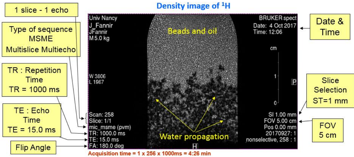
Figure 4.10. MRI vertical slice of a stack of polystyrene beads contained in a PVC tube and initially saturated with oil. The aqueous solution of MnCl_2 is injected from the bottom with a flow rate of 0.12 mL/min. Water saturated regions appear in black and those saturated with oil in grey.
