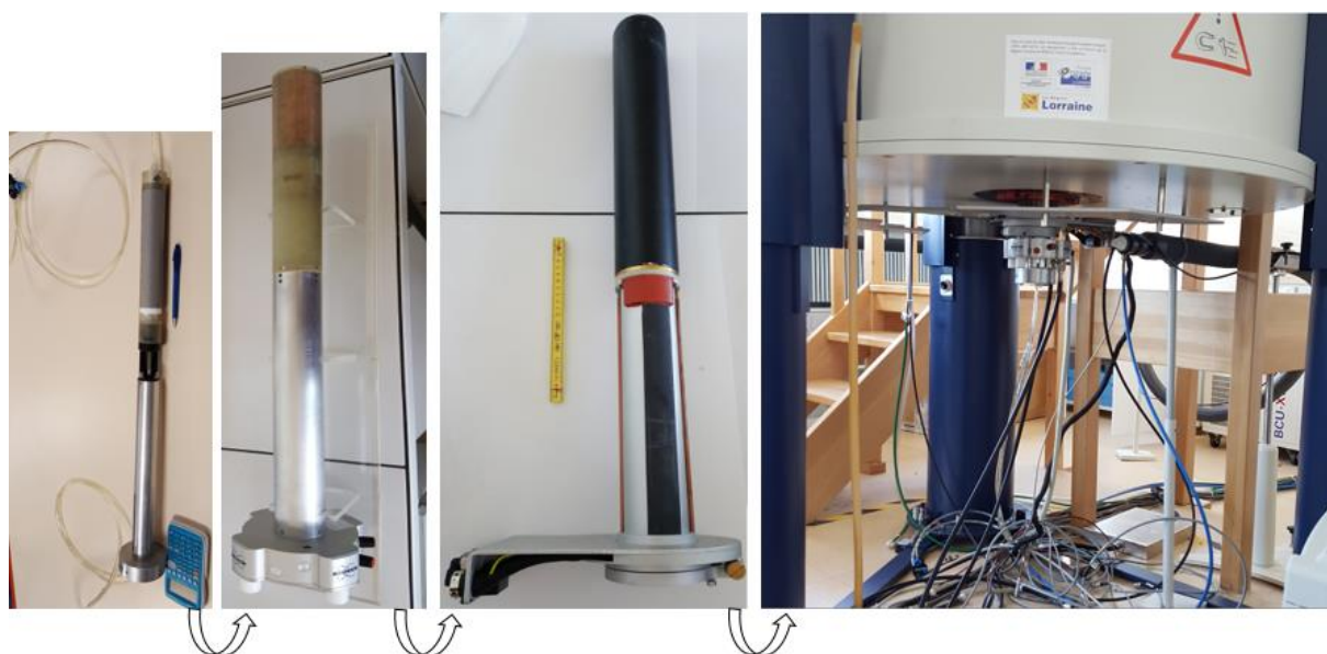
Figure A.2. MRI probe in combination with the Gradient System and the holder with PVC tube sample
