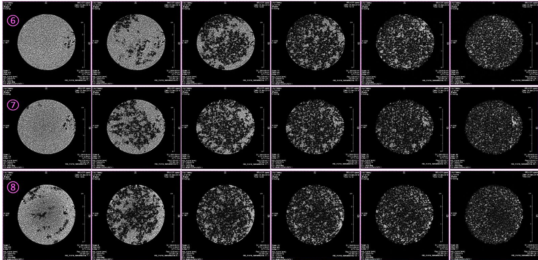
Figure 5.5. Consecutive MR images (ParaVision software) of water–oil displacement in the polystyrene beads model with an injection flow rate of 0.12 mL/min. The lighter areas correspond to those saturated with oil and the darker that gradually appear correspond to areas saturated with water. The acquisition of MRI signal was made each 15 minutes and shown here from the first water appearance in the FOV. The two dotted lines on the vertical images indicate the area of interest, where we can then perform the analysis and calculations. (a) Vertical cross-section. (b) The eight horizontal cross-sections.
