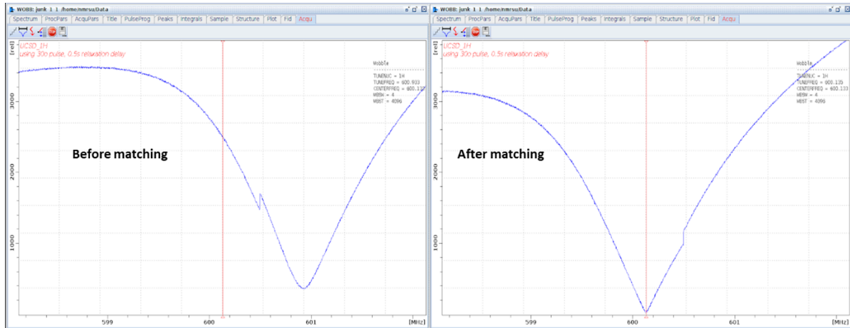
Figure 4.8. Wobble curve, before and after tuning & matching.
