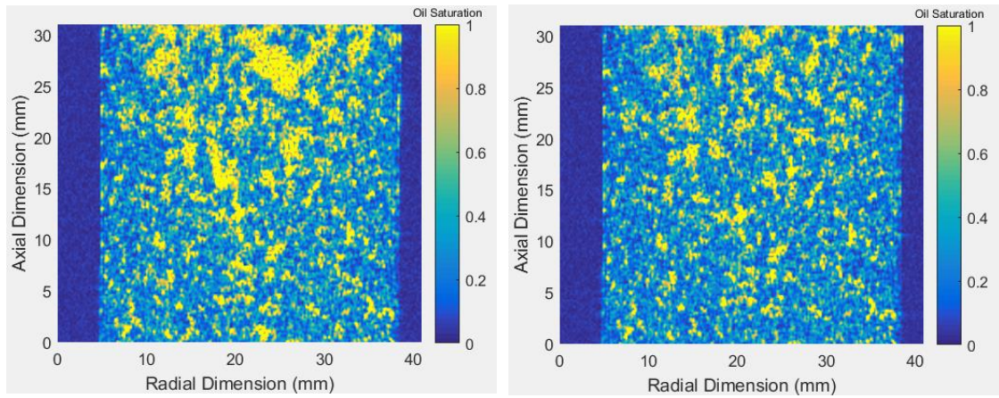
Figure 5.8. Visualization of the two-phase displacement in the long-tube model from the MR images of vertical sections. The oil is yellow and the water is light blue. The acquisition of MRI signal was made each 15 minutes and shown here from the first water appearance in FOV. The last image is the residual oil saturation image, where the oil saturation was stabilized.
