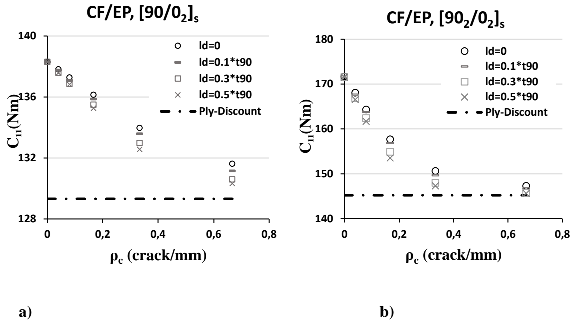
Figure 16: Delamination effect on bending stiffness of CF/EP laminates with cracks in 90°-layer for two different Lay-ups
