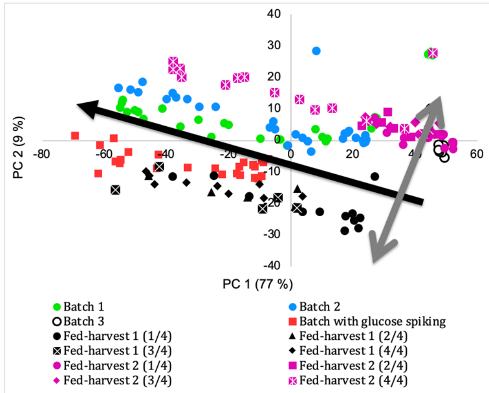
Figure 4.3-1. Calibration spectra set analysis
