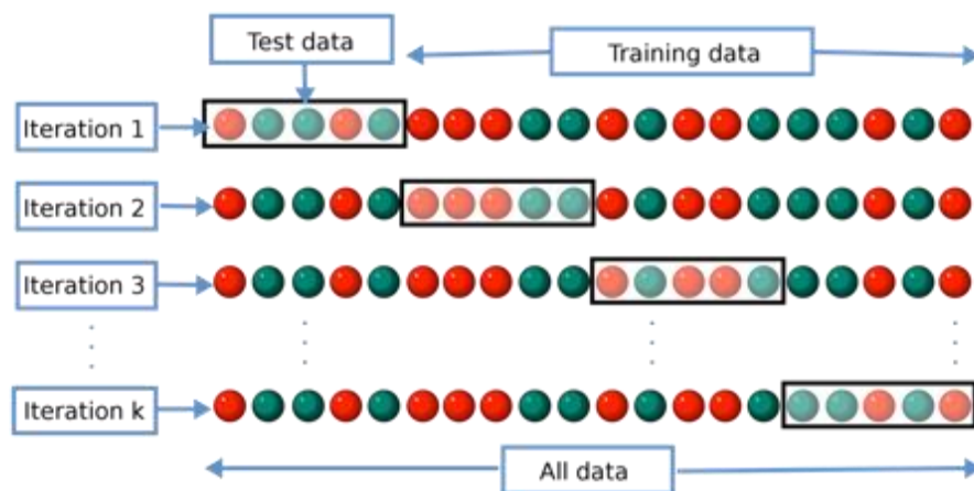
Figure 12. Cross-validation approach
