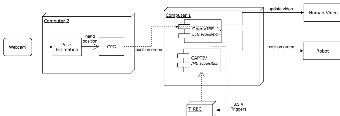
Figure 7.3: Setup for part 2 of the experiment. The setup of part 1 is combined with a second computer which also processes the visual input with a pose estimation algorithm and feeds the hand position into the CPG controller to get the position orders. Robot commands are then transmitted to the first computer which controls the robot
