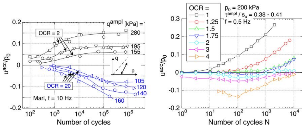
Figure 1.28: Effect of overconsolidation ratio on cyclic behavior. (a) OCR=2-20 (Brown et al. 1975); (b) OCR=1-4 (Matsui et al. 1980). adopted from (Wichtmann et al. 2013).
