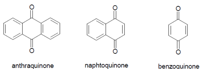
Figure 20. Classification of quinones.
