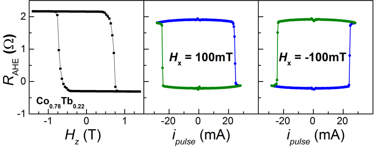
Figure 4.7: (a) Field - induced magnetization switching, measured with AHE, R_{\text{AHE}}(H_z) cycle and (b),(c) current-induced magnetization switching using ( H_x = \pm 100 mT) for sample \text{Si-SiO}_2/\text{W}(3)/\text{Co}_{0.78}\text{Tb}_{0.22}(3.5)/\text{Al}(3) . This is a Co-rich sample at room temperature, close to the compensation point.
