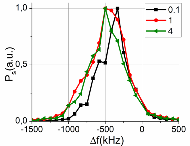
Figure 9.13: Power spectra probing at antenna vertical shift +2cm. Different lines correspond to different amplitudes of the turbulence.
