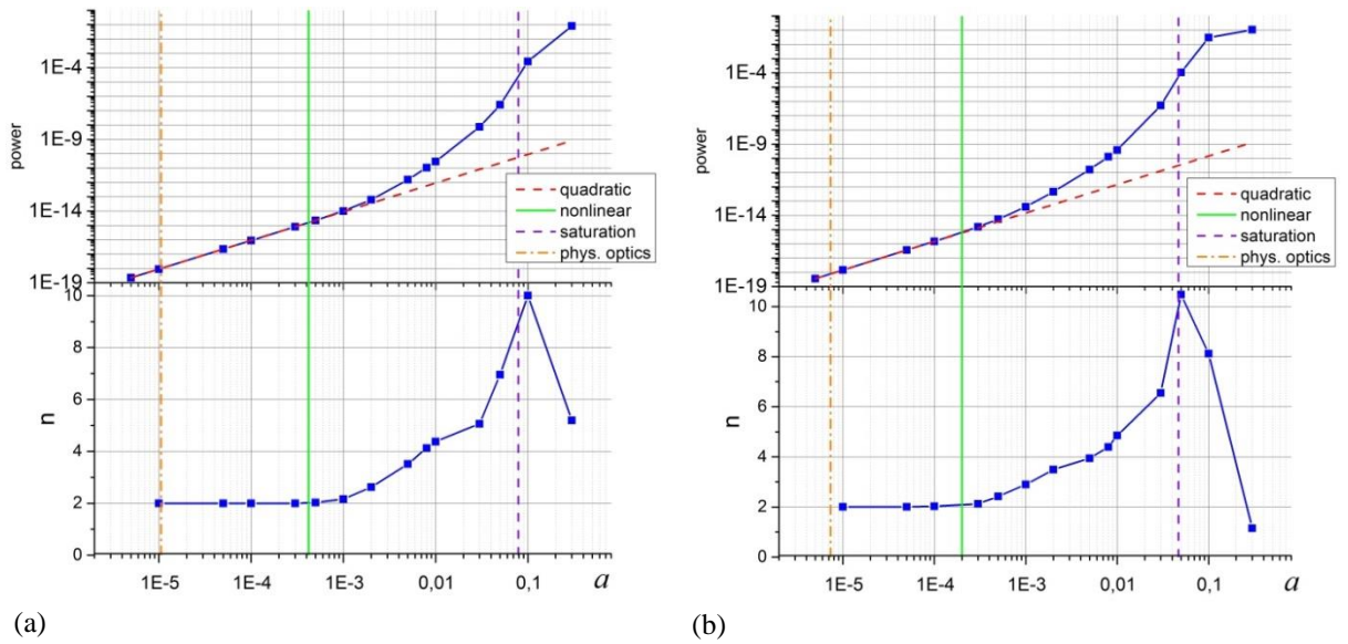
(a) (b) Figure 8.4. Scattered signal power and its exponential scaling calculated in case of radially uniform turbulence depending on turbulence amplitude a for (a) l_{cy}=1.3 cm and the probing angle \vartheta=40^\circ and for (b) l_{cy}=1.3 cm and the probing angle \vartheta=30^\circ . The dashed red line corresponds to quadratic power dependence. Vertical lines correspond to nonlinearity thresholds: solid green line - our analysis, formula (8.19b); orange dash-dotted line - physical optics, formula (8.19a); purple dashed line -saturation, formula (8.25a).
