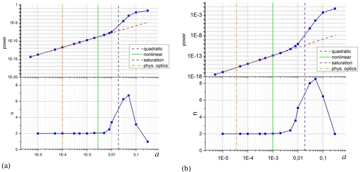
(a) (b) Figure 8.5. Scattered signal power and its exponential scaling depending on turbulence amplitude a in case of 2D turbulence with (a) l_{cx}=l_{cy}=1.3 cm and (b) l_{cx}=l_{cy}=1.2 cm. The dashed red line corresponds to quadratic
