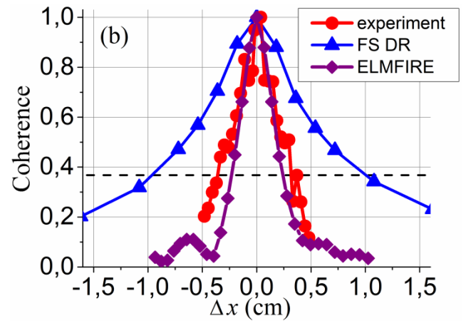
Figure 9.7b: The RCDR CCF against the turning point radial separation. Triangles – fast synthetic DR; circles – experiment; diamonds – turbulence CCF computed directly from ELMFIRE.
