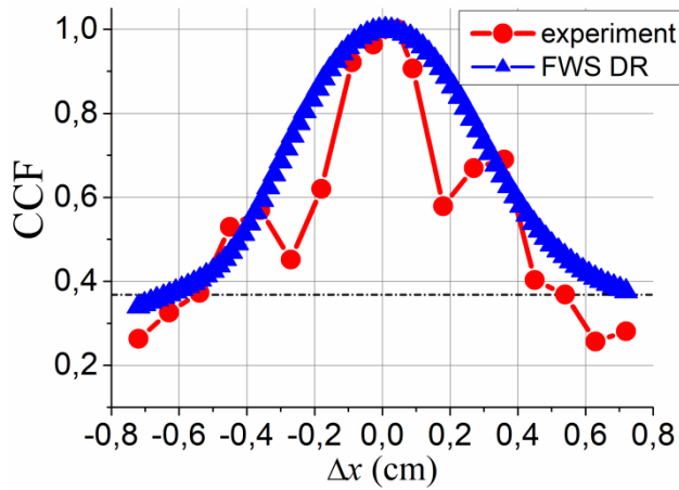
Figure 9.18: RCDR CCF determined experimentally and calculated with a synthetic diagnostic for -2.3 cm antenna.
