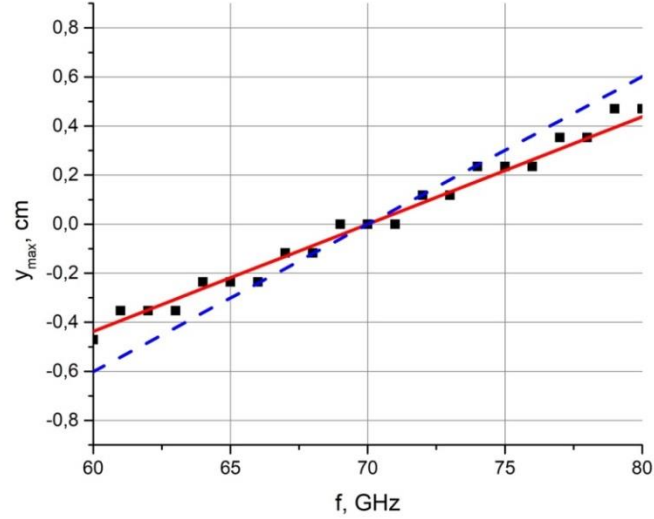
Figure 7.5: Dependence of y_{max} on the probing frequency. L=4 cm, l_{min}=0.2 cm, l_{max}=1.4 cm, \rho=1.6 cm, \gamma=45^\circ , f=70 GHz. Black symbols correspond to numerical evaluations, solid red and dashed blue lines are given by formula (7.14) and “heuristic” interpretation given in [50] respectively.
