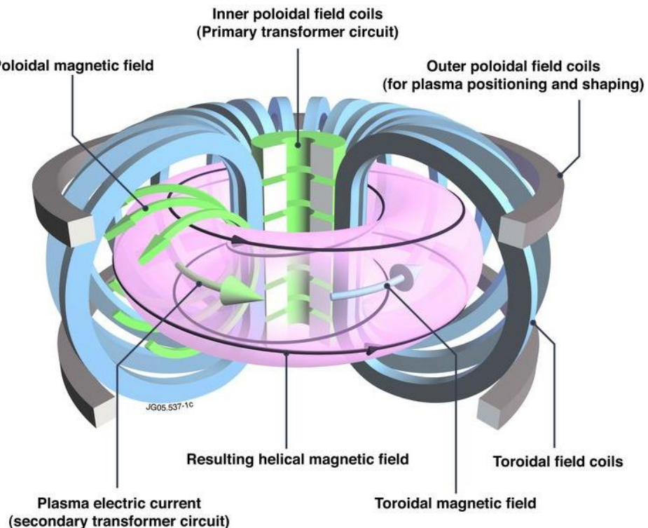
Figure 1.2. The scheme of a typical tokamak device. Sourced from [8].
