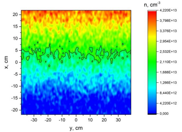
Figure 8.3: 2D density profile with random fluctuations. Grey line designates cut-off density for the probing frequency used in FD3D calculations.
