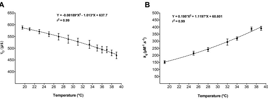
Figure 4. Temperature dependencies of \tau_0 and k_q of the Pd-TCPP-albumin complex maintained at a constant pH of 7.4.
