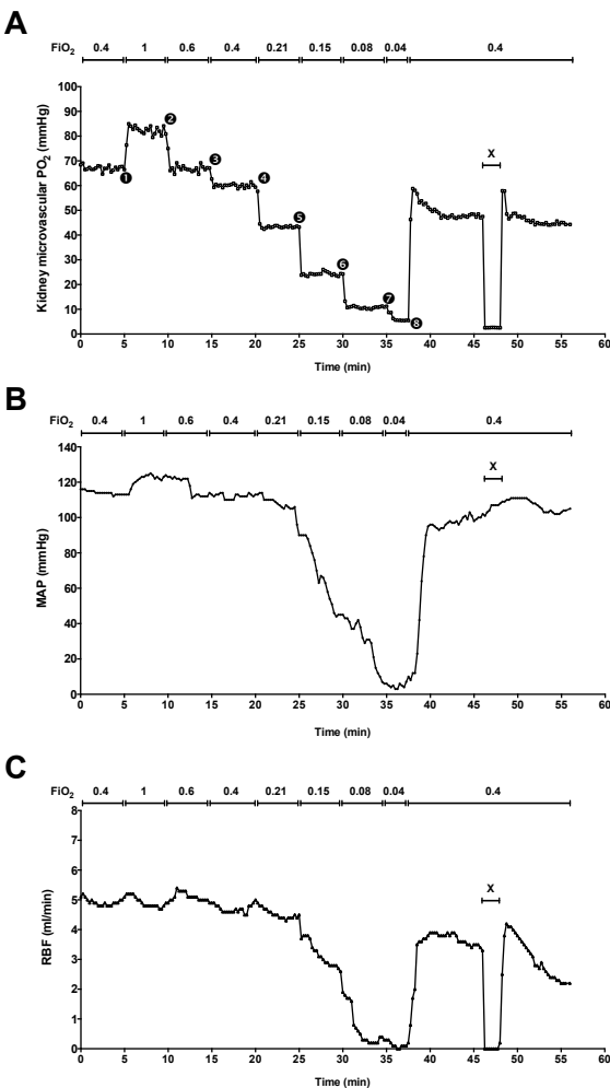
Figure 7. Typical example of renal microvascular PO 2 and macrohemodynamic trends during hypoxic ventilation and ischemia.
