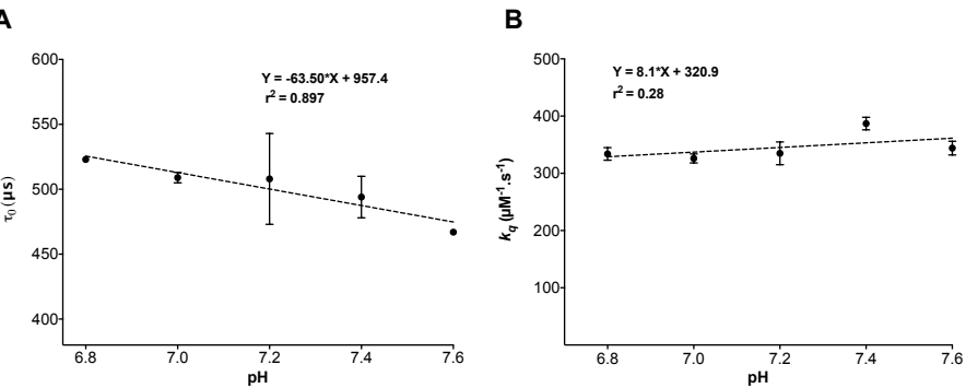
Figure 5. pH dependency of \tau_0 and k_q with temperature kept constant at 37°C
