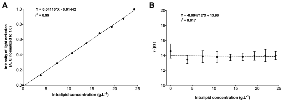
Figure 6. Decay times plotted against lipid emulsion concentrations
