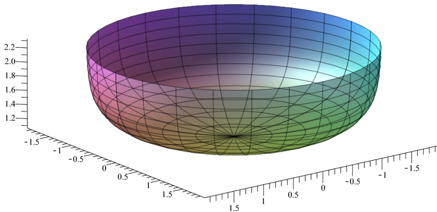
Figure 4 – CMC disk type surface D_H^2 in \mathbb{H}^2 \times \mathbb{R} with H = 1/8 :
