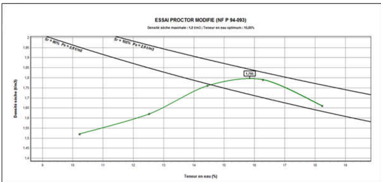
Figure 22 : Courbe Proctor
