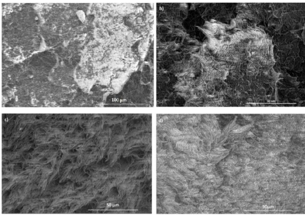
Fig. 10. Evolution of the fracture surfaces of a) unmodified CA 100, b) 0.5:1, c) 1:1, and d) 1.5:1 materials by SEM micrographies.
