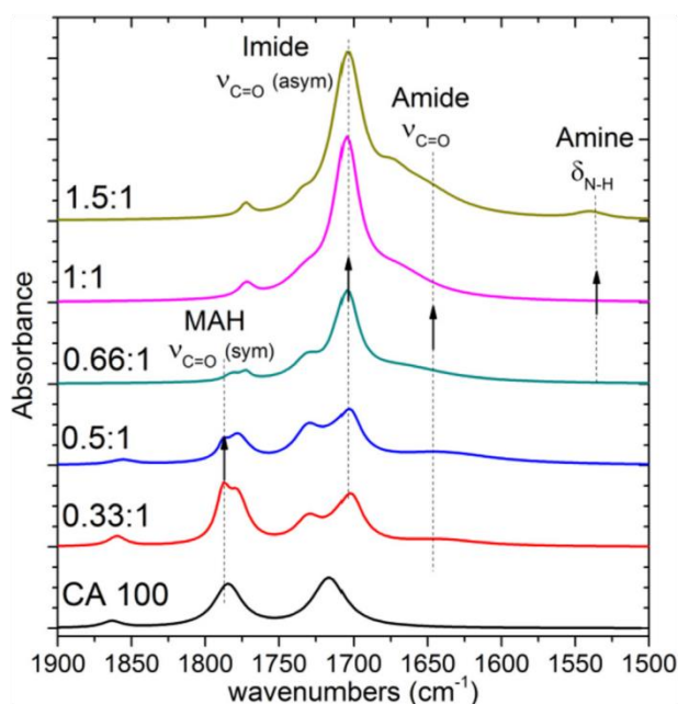
Fig. 4. Evolution of the FTIR spectra as a function of the MAH: \text{NH}_2 molar ratio.
