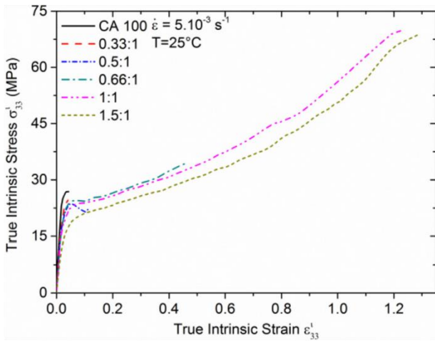
Fig. 11. True intrinsic mechanical behaviours of the different materials as function of the \text{NH}_2 :MAH molar ratio.
