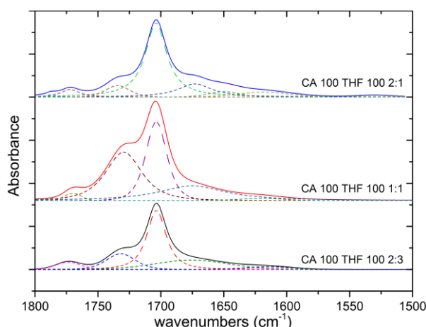
Figure II.6: Spectre FTIR des fractions insoluble des matrices réticulées
