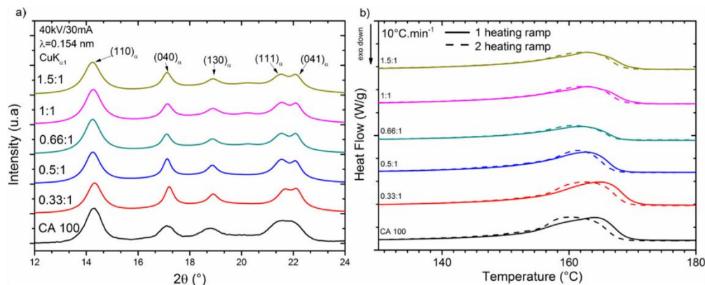
Fig. 5. a) 1D WAXS diffractograms and b) DSC thermograms evolution as a function of the \text{NH}_2 :MAH molar ratio.
