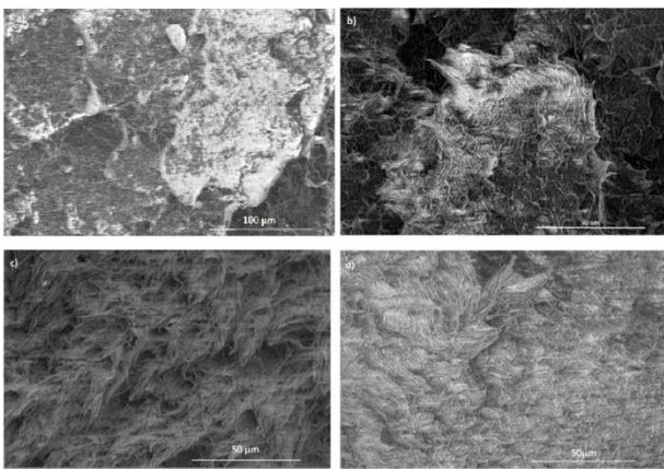
Fig. 10. Evolution of the fracture surfaces of a) unmodified CA 100, b) 0.5:1, c) 1:1, and d) 1.5:1 materials by SEM microographies.
