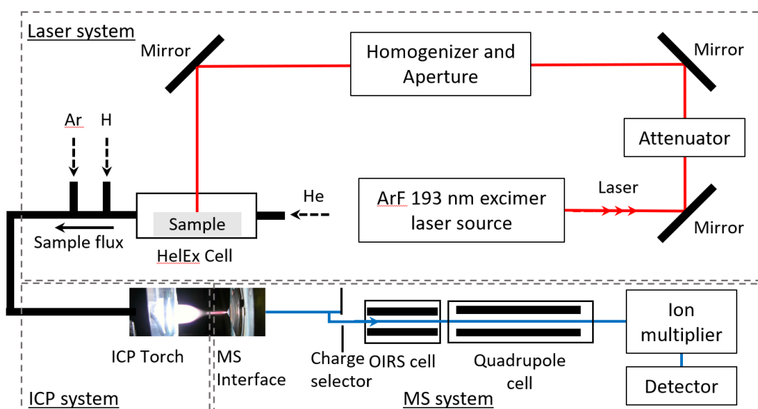
Figure 2.4: Representation of the major component of a LA-ICP-MS. The red line is the laser and the blue line is the ion beam after the plasma in the mass spectrometer.
