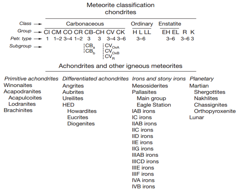
Figure 1.1: Meteorites classification after Krot et al. (2014).
