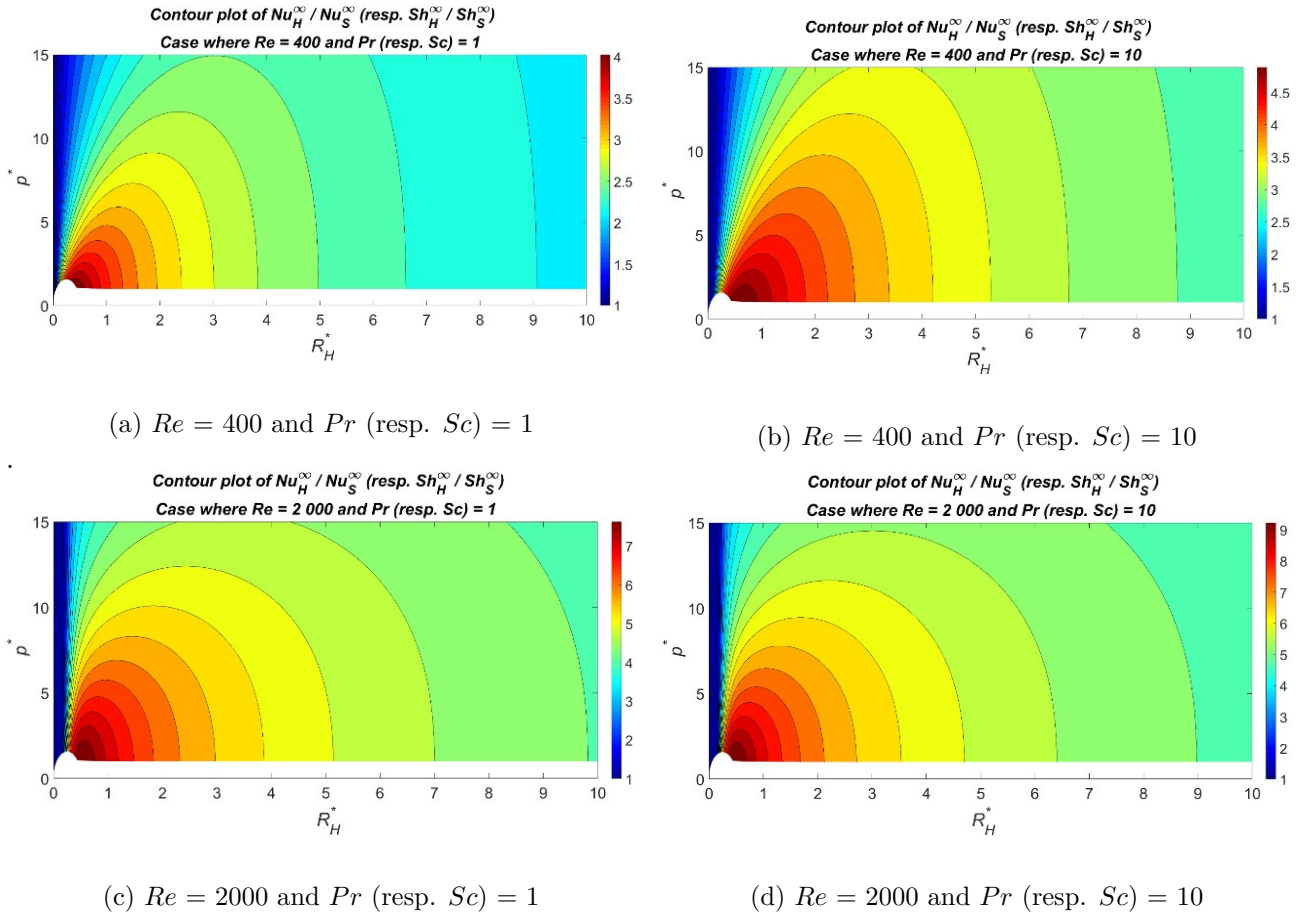
Figure 3.9: Contour plots of the Nu_H^\infty to Nu_S^\infty (respectively Sh_H^\infty to Sh_S^\infty ) ratio calculated using the present correlation (Eqs. 3.13). The contour plots at Re = 400 were generated using the set of parameters valid for 10 \leq Re \leq 400 (Table 3.2)
