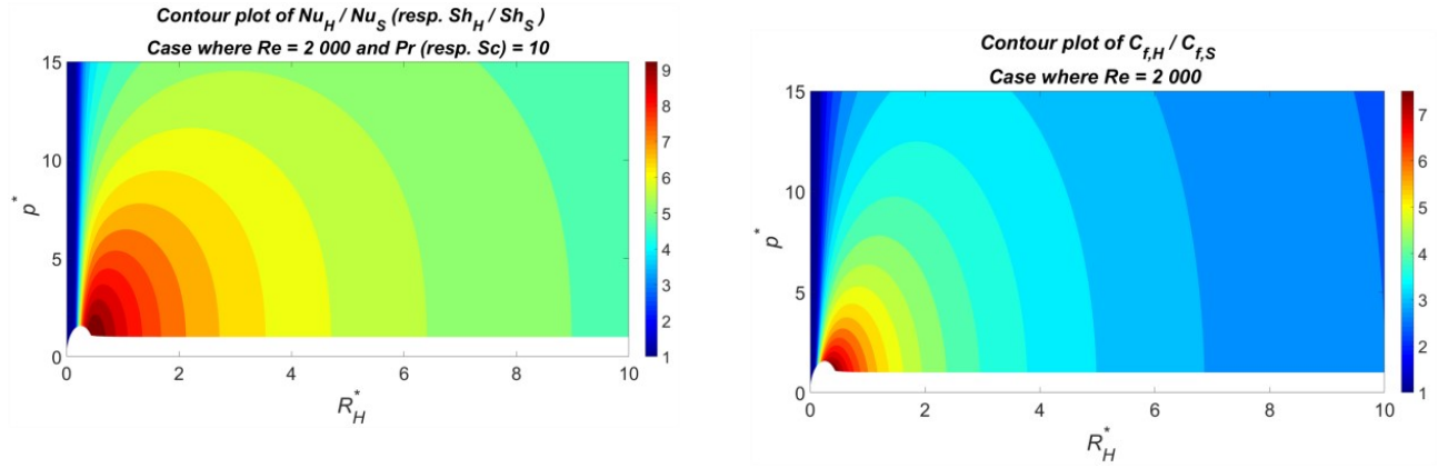
(a) The Nu_H to Nu_S (respectively Sh_H to Sh_S ) ratio, as calculated using the correlations of Abushammala et al.(2020) [208]
