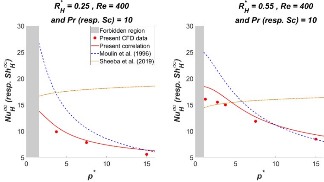
Figure 3.11: Nu_H^\infty (respectively Sh_H^\infty ) versus p^* at two different R_H^* : comparison between the present correlation and those of Moulin et al. (1996) [168] and Sheeba et al (2019) [220]
