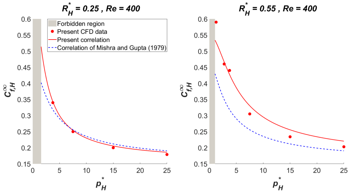
Figure 2.13: C_{f,H}^{\infty} versus p_H^* at two different R_H^* : comparison between the present correlation and that of Mishra and Gupta (1979) [194]
