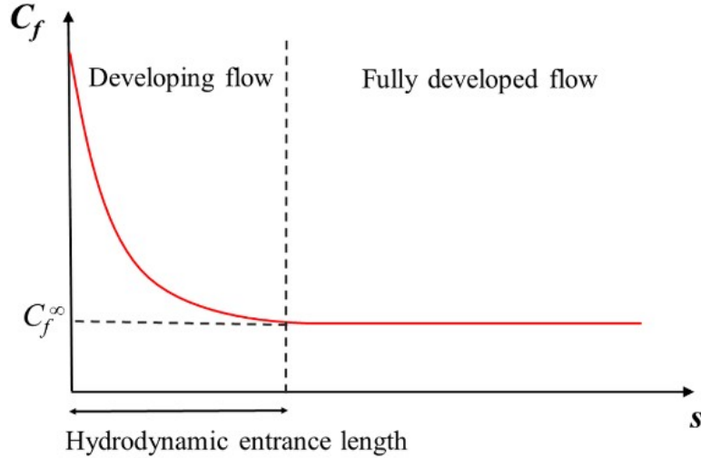
Figure 2.5: Typical variation of the friction factor from the entrance of a straight or a helical pipe
