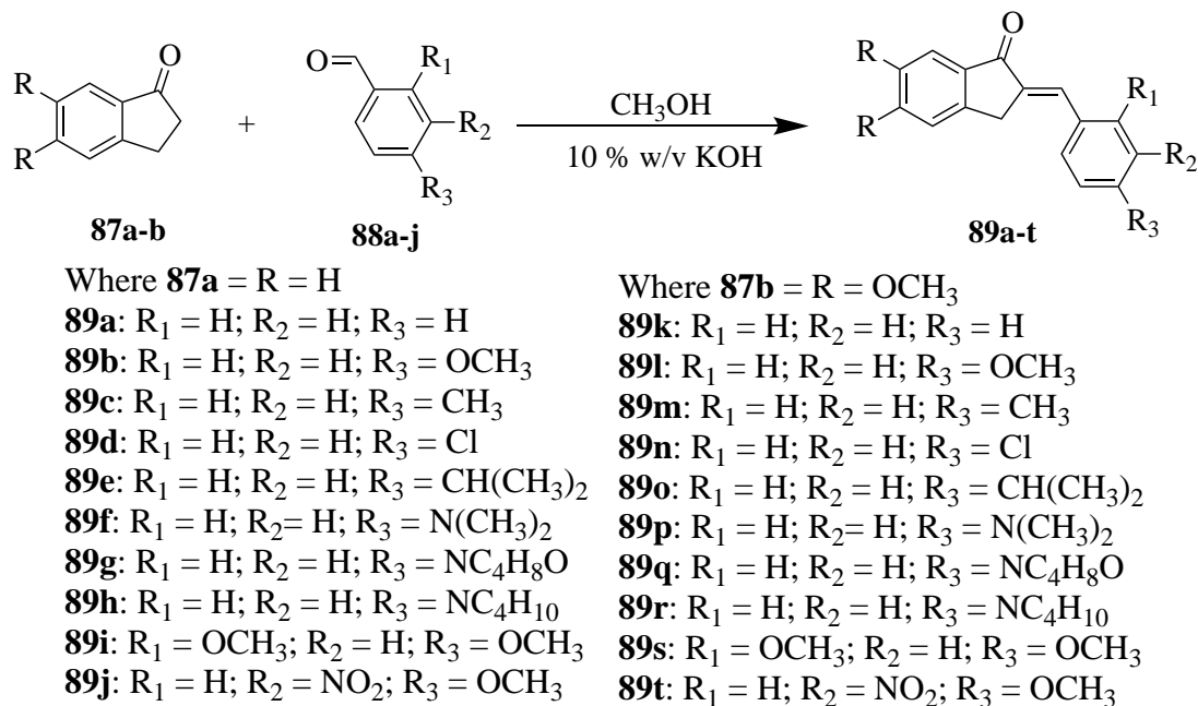
Scheme 3.4: The synthesis of benzylidene indanone derivatives.
