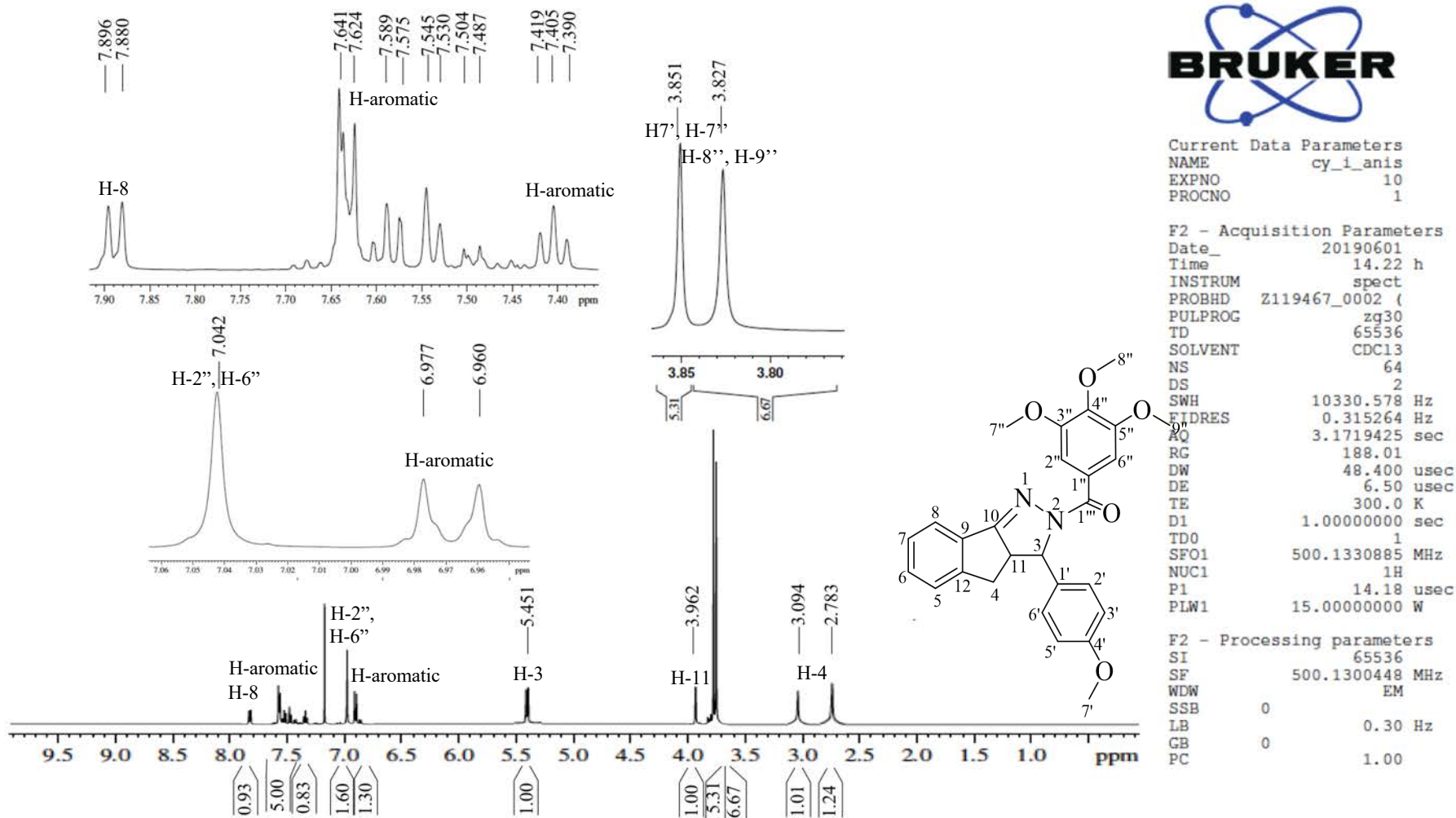
Figure 4.23: The 1 H NMR spectrum for compound 90b
