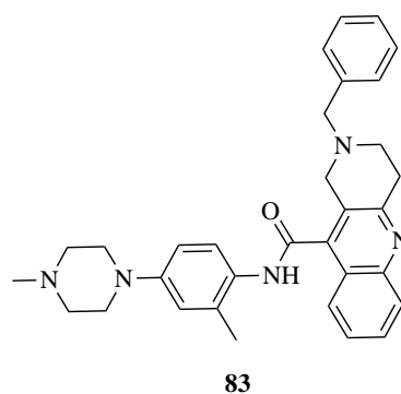
Figure 2.14: The structure of compound 83
