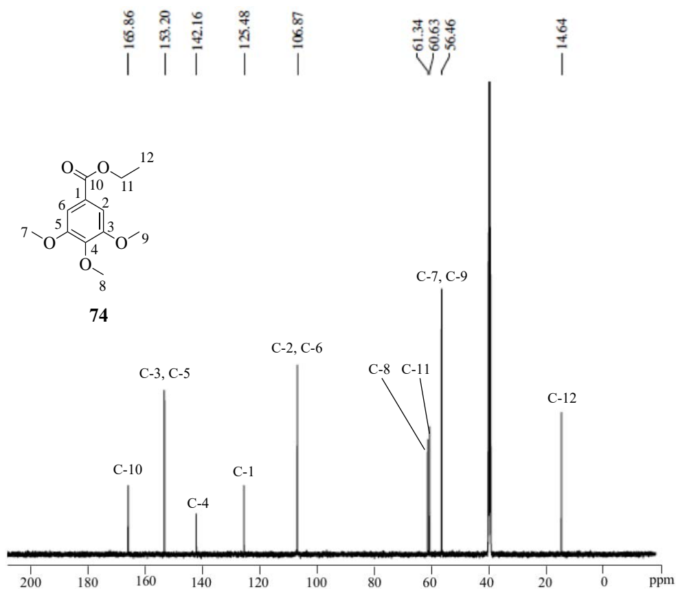
Figure 4.8: The 13 C NMR spectrum of compound 85
