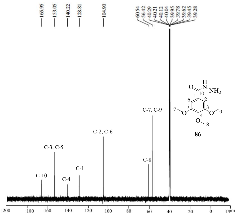
Figure 4.12: The ^{13}\text{C} -NMR spectrum of compound 86
