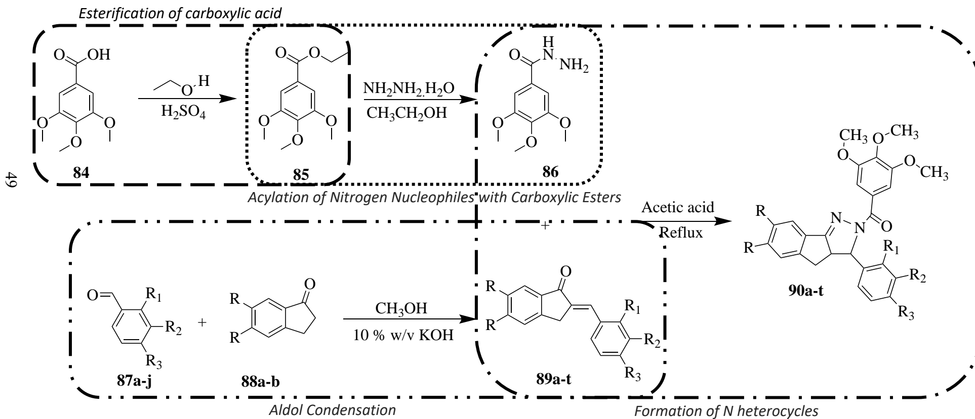
Scheme 3.1: The synthesis of pyrazolyl substituted benzylidene indanone derivatives
