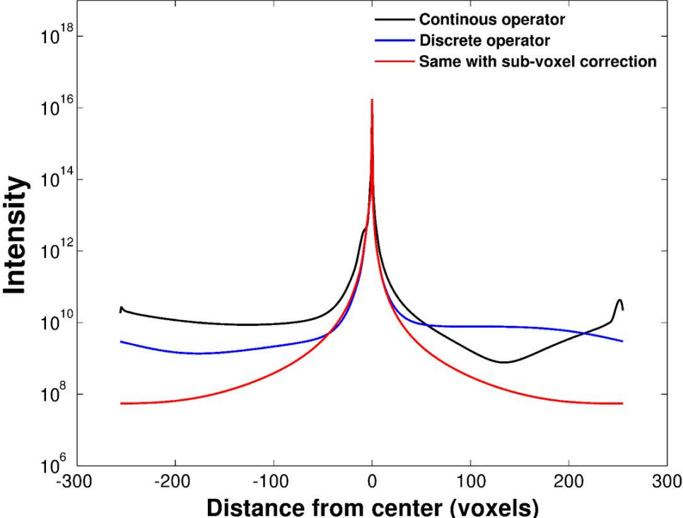
FIGURE 4.9 – 1D peak profiles computed for one dislocation loop using the different methods described in the previous chapter
