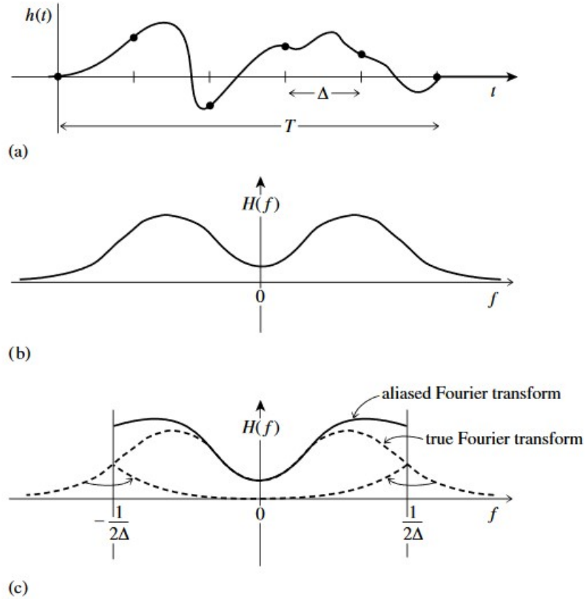
FIGURE 1.34 – The continuous function shown in (a) is nonzero only for a finite interval of the period T . It follows that its Fourier transform, whose modulus is shown schematically in (b), is not bandwidth limited but has finite amplitude for all frequencies. If the original function is sampled with a sampling interval \Delta , as in (a), then the Fourier transform (c) is defined only between plus and minus the Nyquist critical frequency. Power outside that range is folded over or "aliased" into the range. The effect can be eliminated only by low-pass filtering the original function before sampling
