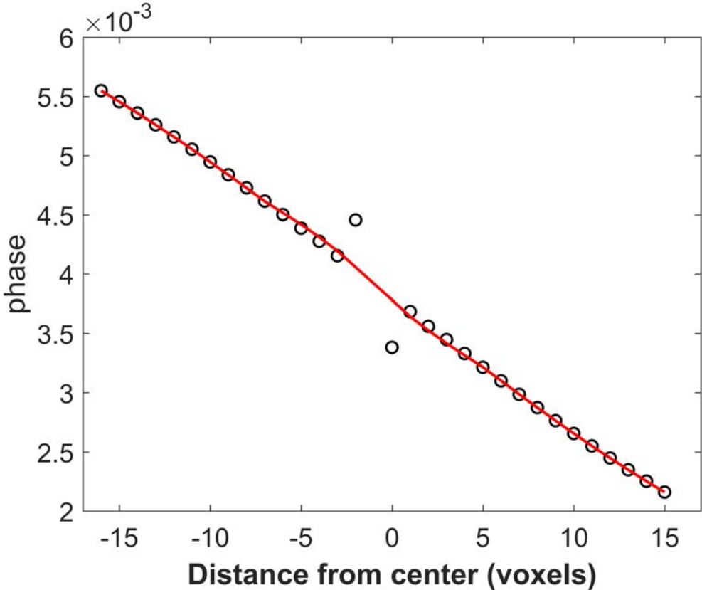
FIGURE 3.8 – Local oscillation of the phase due to artifacts (the representation is made for 32 voxels centered in the unit cell along z direction). The red line is approximately equal to the phase expected for this displacement field
