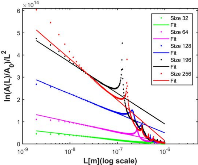
FIGURE 4.21 – Normalized real part \ln(A_L/A_0)/L^2 of the FFT of the peaks for the (200) \mathbf{g} vector for 64 random distribution of hexagonal loops with the same voxels side : 32, 64,128, 196, 256 voxels configurations are represented.
