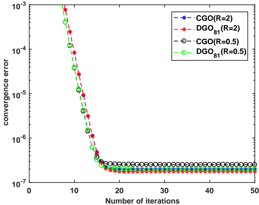
FIGURE 2.15 – The convergence error computed with the strain field criterion for both CGO and DGO_{81} methods as a function of iteration number up to 50 iterations for two mechanical contrasts : R = K_m/K_i = 2 and R = K_m/K_i = 0.5 .
