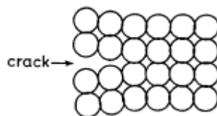
Figure 2-8 Agglomerate fracture model according to Kendall (1988)
