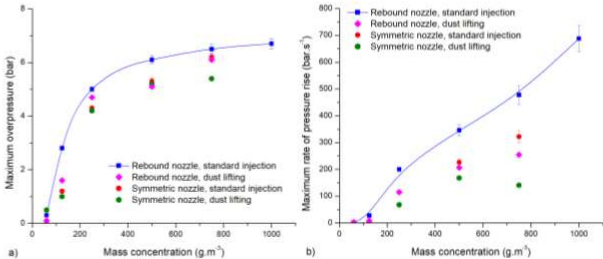
Figure 5-27 Evolution of the a) overpressure and b) rate of pressure rise of aluminum 100 nm for various injection procedures
