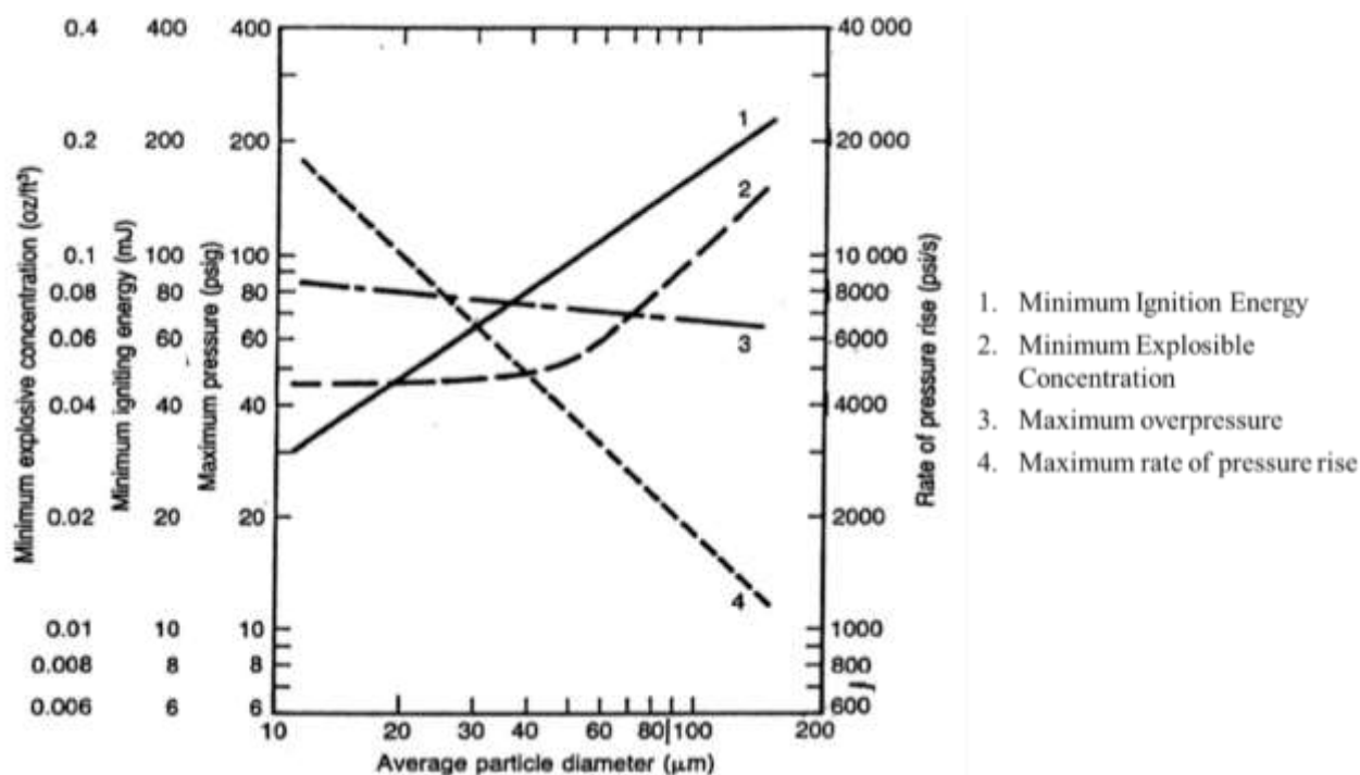
Figure 2-3 Explosion characteristics as a function of aluminum particle size (Baudry, 2007; Jacobson et al., 1964; Nagy and Verakis, 1983)
